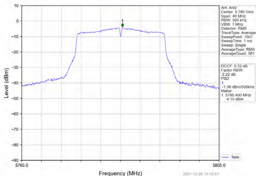
802.11n(HT20)_MCH_5785MHz_MIMO_NTN
