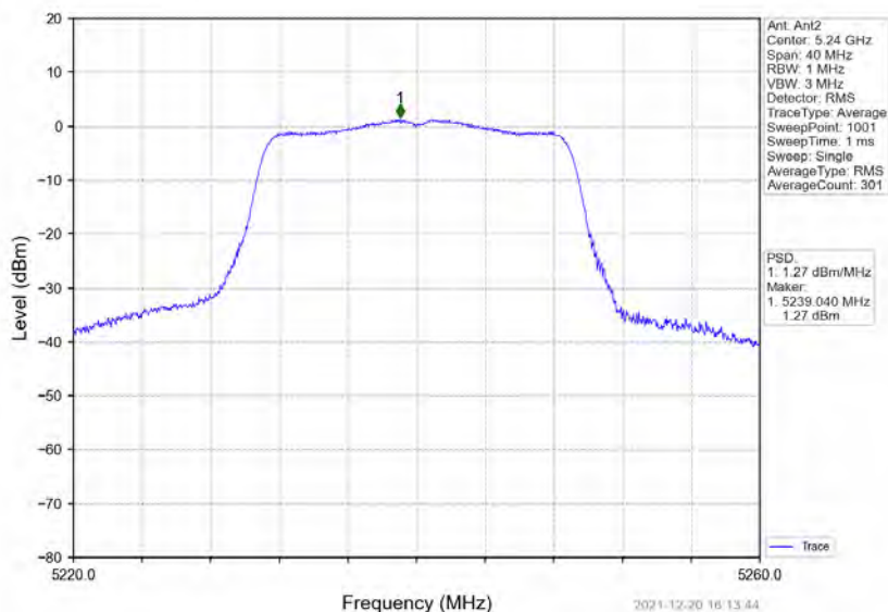
802.11ac(VHT20)_HCH_5240MHz_MIMO_NTNV
