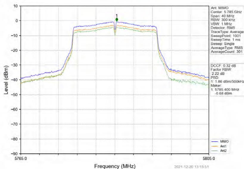
802.11n(HT20)_MCH_5785MHz_MIMO_NTN
