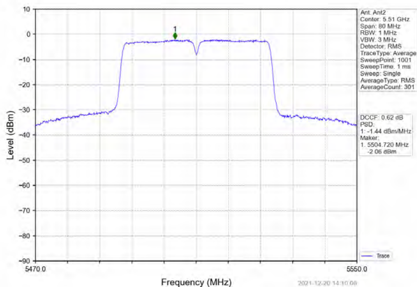
802.11n(HT40)_LCH_5510MHz_MIMO_NTNV
