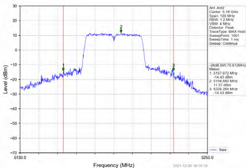
802.11ac(VHT40) LCH_5190MHz_Ant2_NTNV
