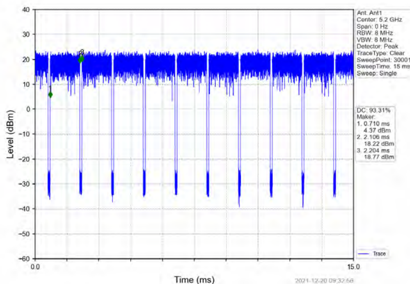
802.11a_HCH_5240MHz_Ant1_NTNV
