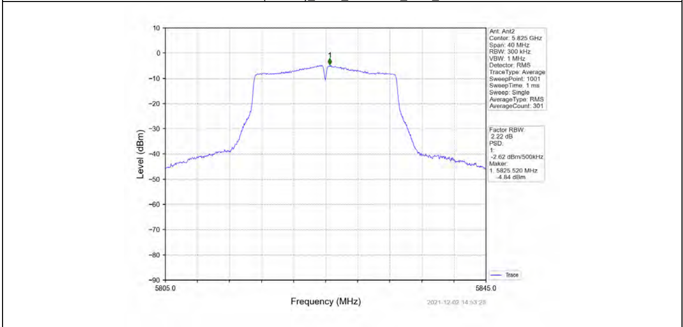
802.11ac(VHT20)_HCH_5825MHz_MIMO_NTNV
