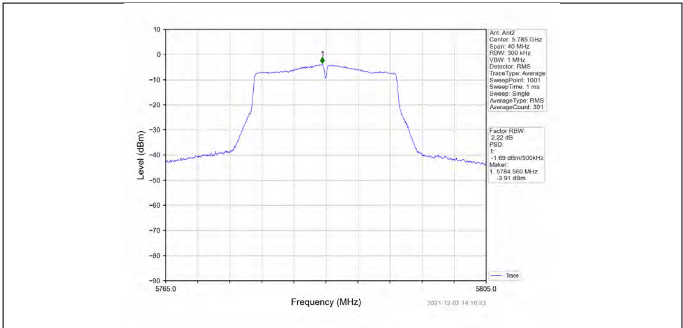
802.11ac(VHT20)_MCH_5785MHz_MIMO_NTNV
