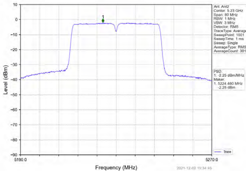
802.11ac(VHT40)_HCH_5230MHz_Ant2_NTNV
