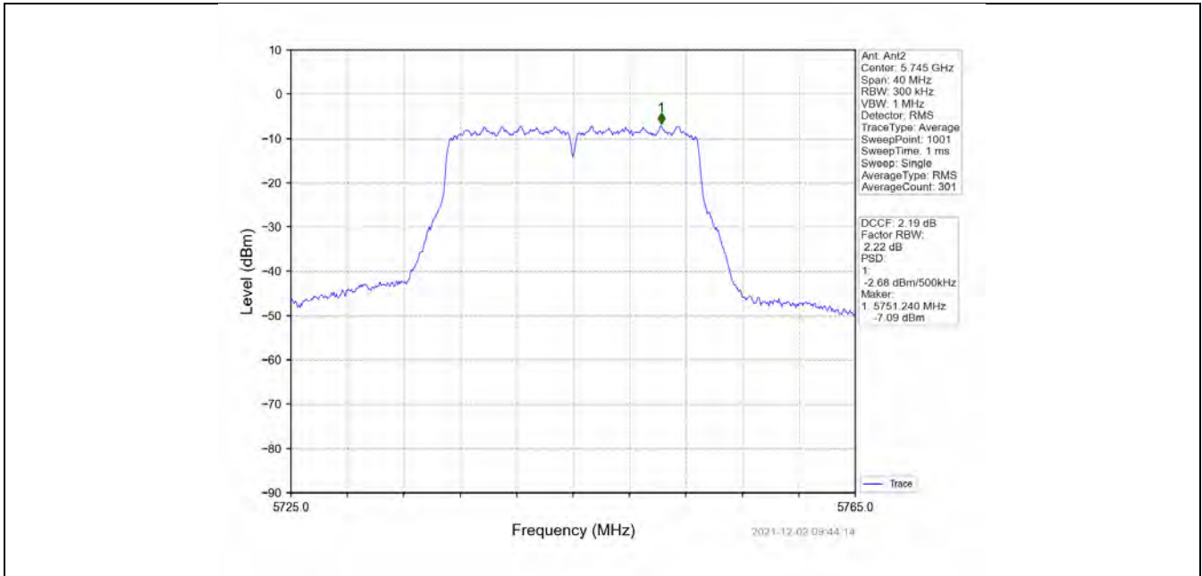
802.11n(HT20)_LCH_5745MHz_MIMO_NTNV
