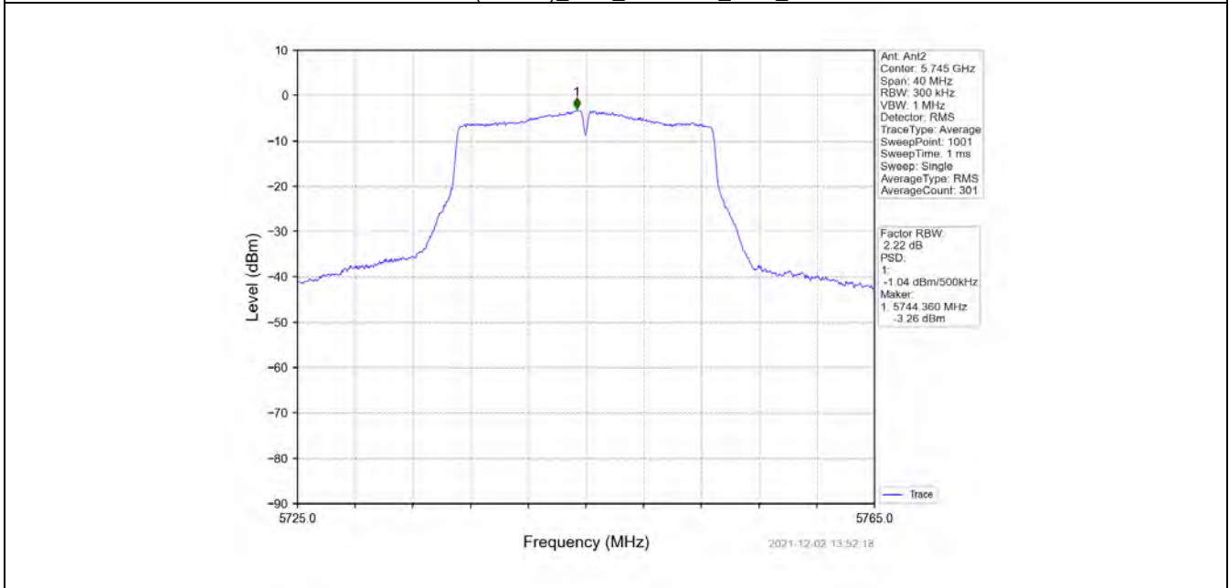
802.11ac(VHT20)_LCH_5745MHz_MIMO_NTNV
