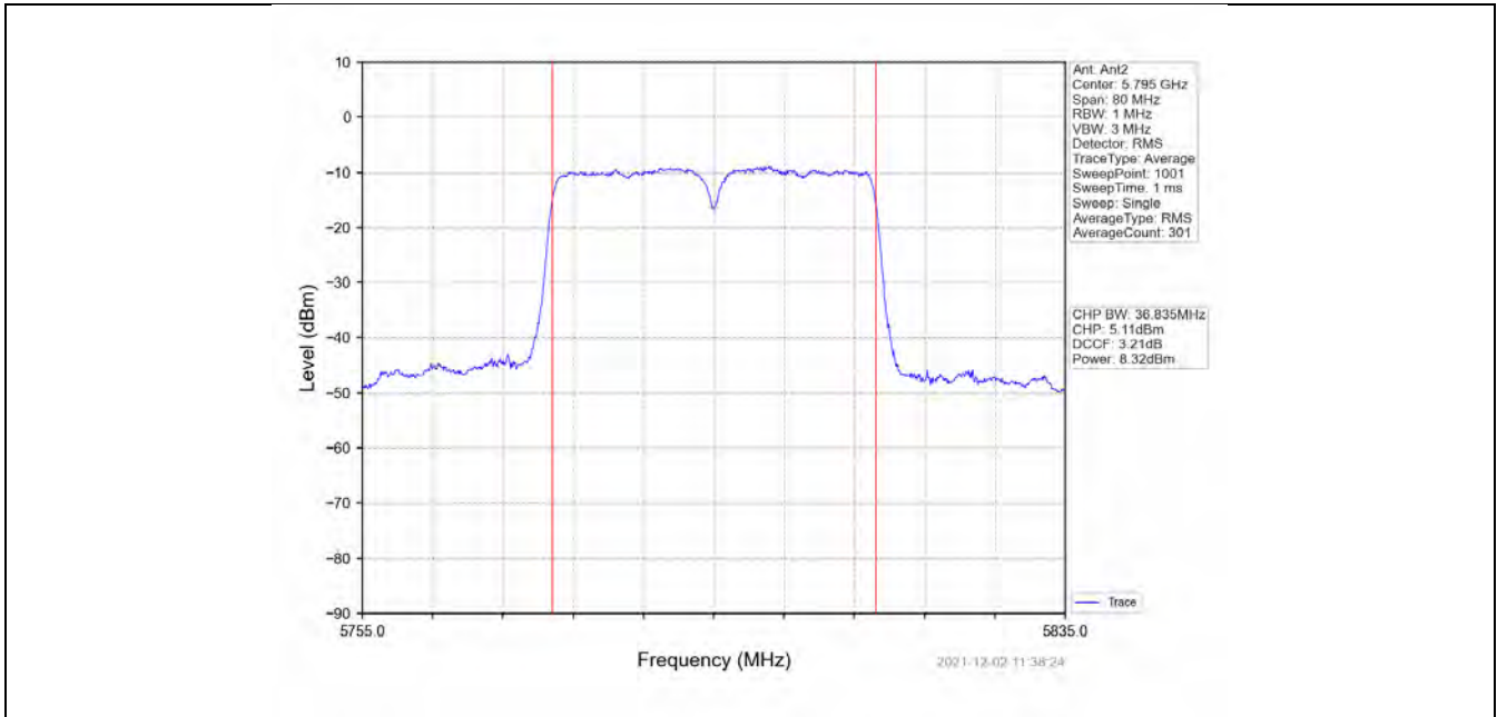
802.11ac(VHT20)_LCH_5180MHz_Ant1_NTNV
