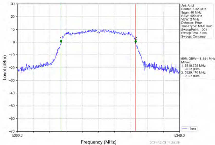
802.11ac(VHT20)_HCH_5320MHz_Ant2_NTNV
