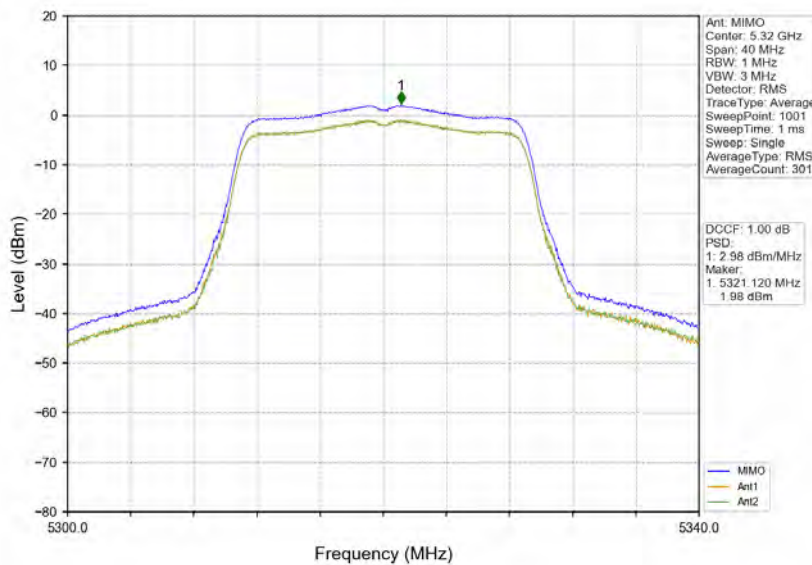
802.11ac(VHT20)_HCH_5320MHz_MIMO_NTNV
