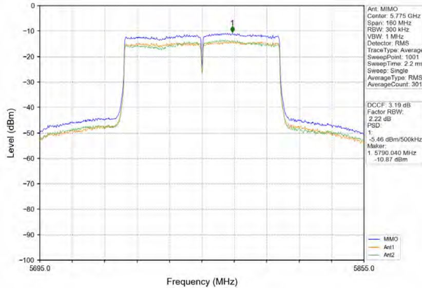
802.11ac(VHT80)_MCH_5775MHz_MIMO_NTNV
