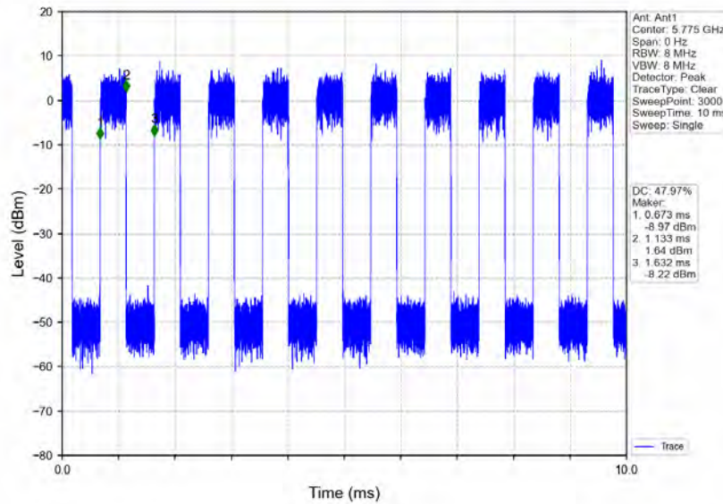
802.11ac(VHT80)_MCH_5775MHz_Ant1_NTNV
