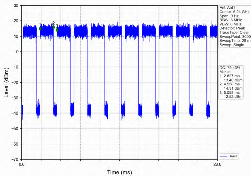
802.11ac(VHT20)_HCH_5240MHz_Ant1_NTNV
