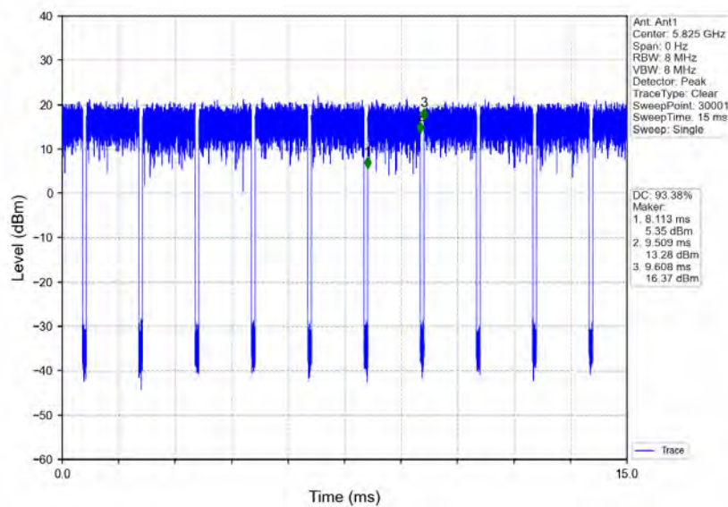
802.11a_HCH_5825MHz_Ant1_NTNV
