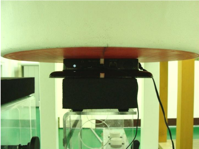
Backside of the DUT with Phantom 0 cm Gap
