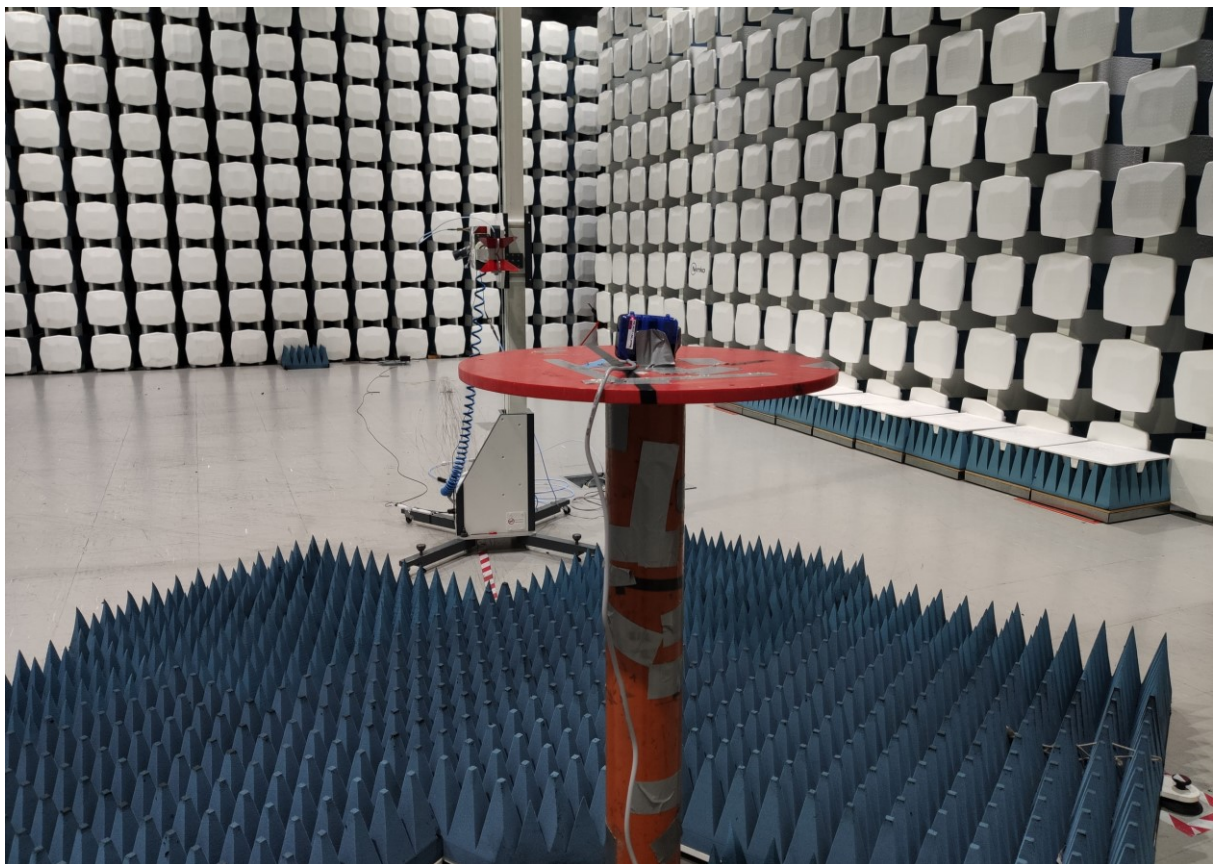
Radiated Emissions, Above 1 GHz
