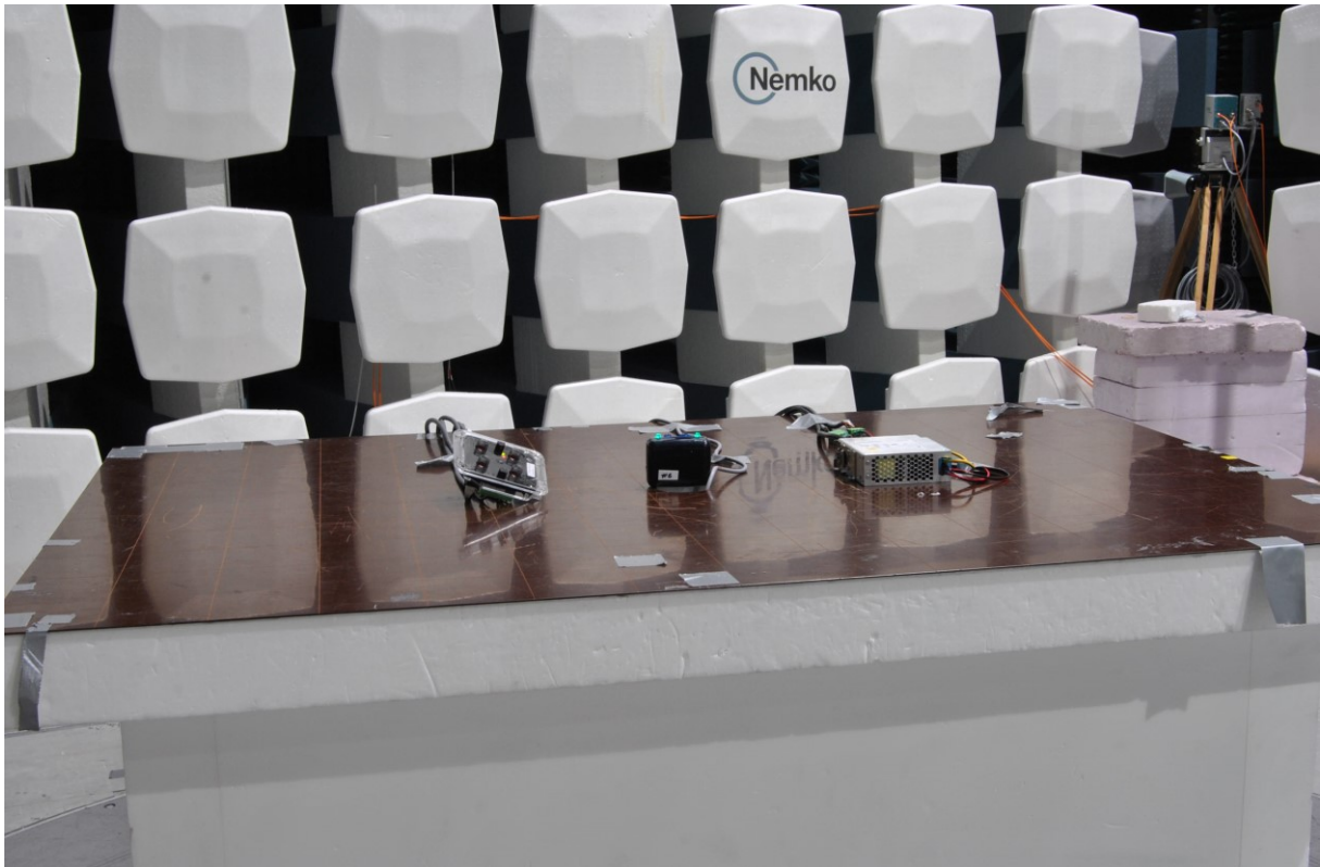
Radiated Emissions, Below 1 GHz
