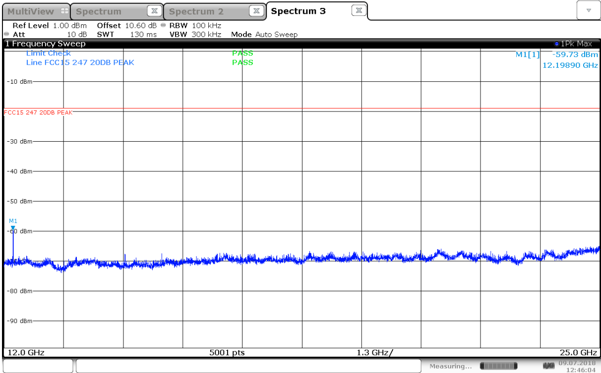
Conducted Emissions, 12000 – 25000 MHz, 2440 MHz
