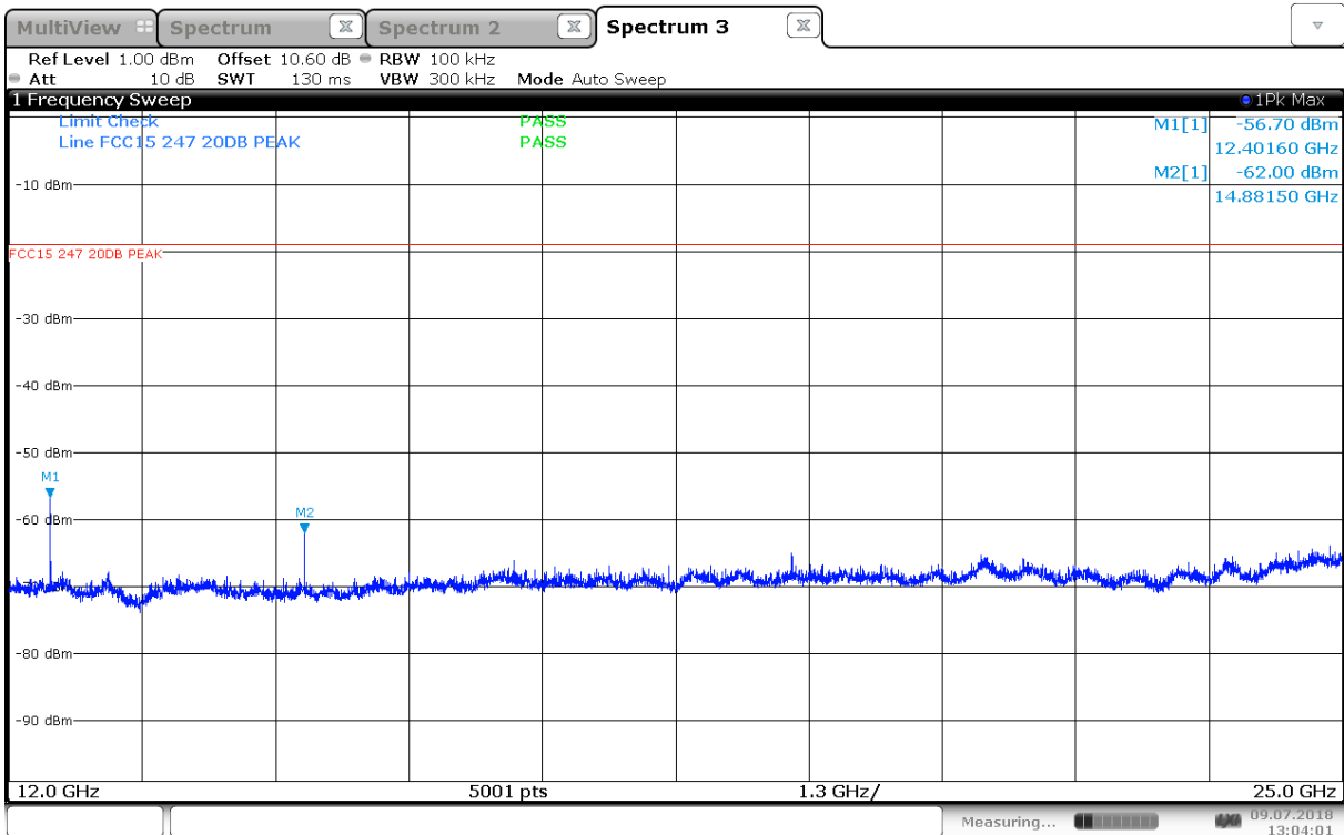
Conducted Emissions, 12000 – 25000 MHz, 2480 MHz
