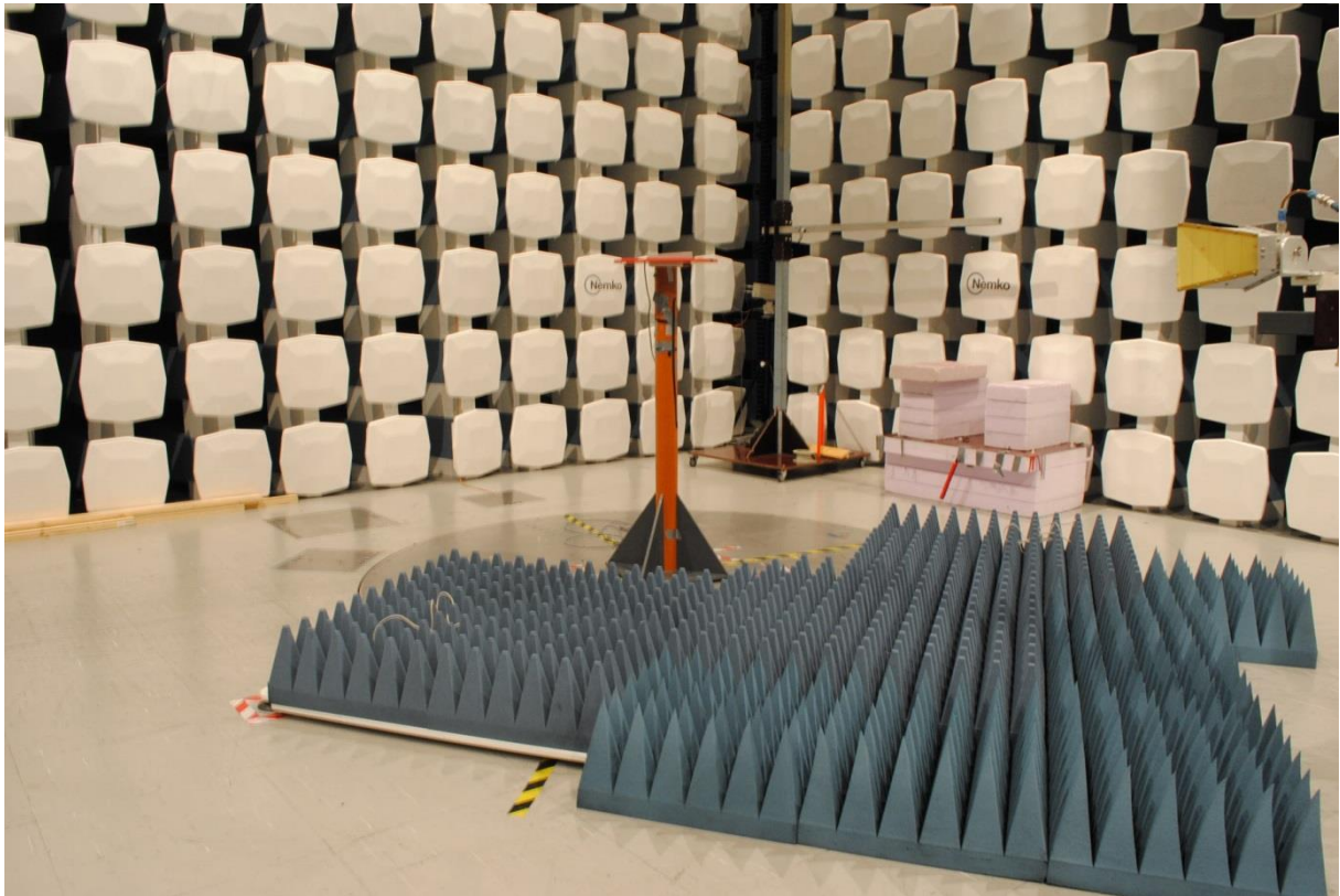
Radiated measurements above 1GHz
