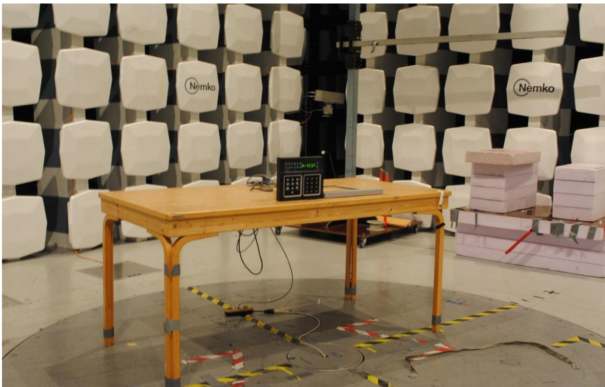
Radiated measurements at 10m - < 30MHz (multi rod reader alone and together with MPC860)
