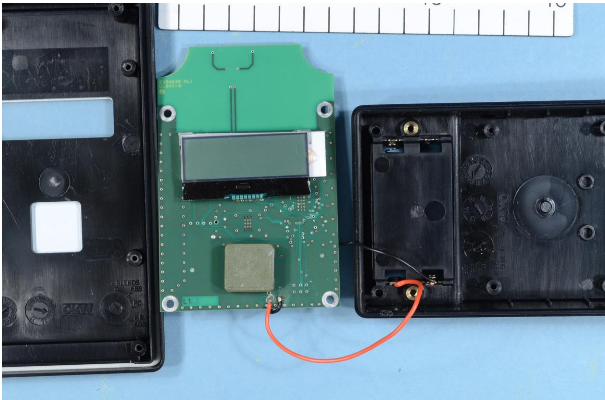
Activity Meter 2 Tester – PCB front & rear view
