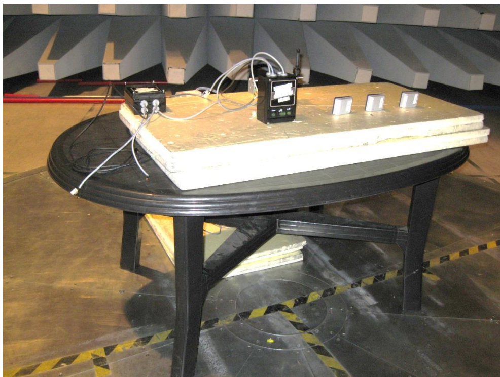
Test setup regarding measurement of radio frequency electromagnetic field < 1 GHz.
