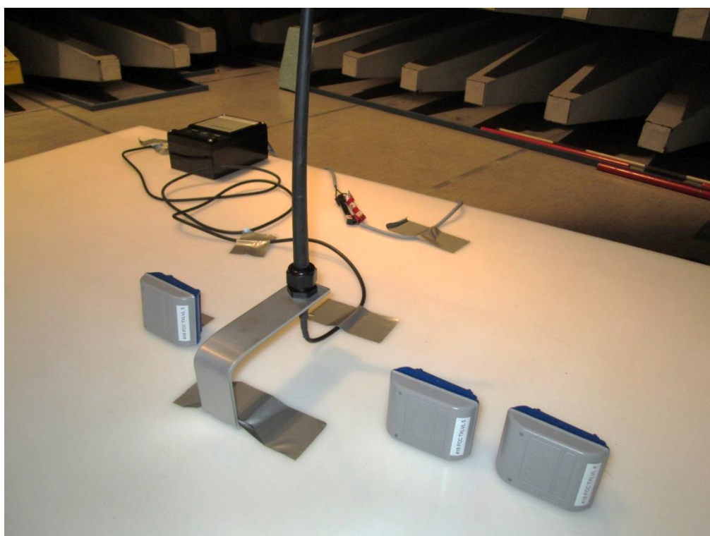
Test setup regarding measurement of peak output field strength of fundamental.
