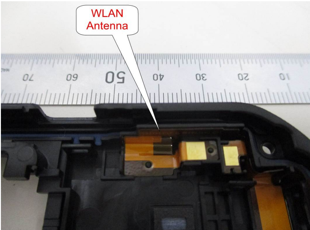
BT / WLAN Main Antenna
