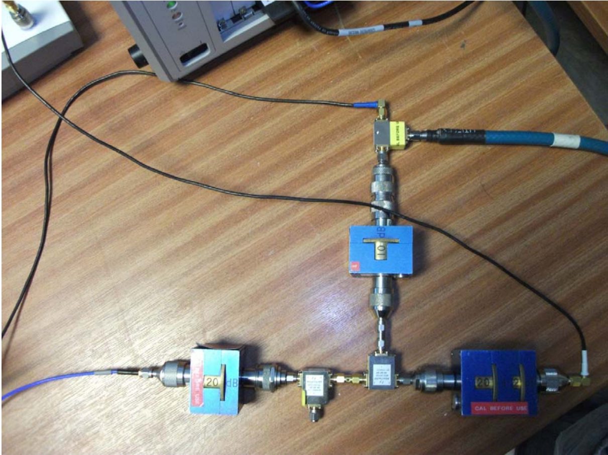
Test Attenuation Network
