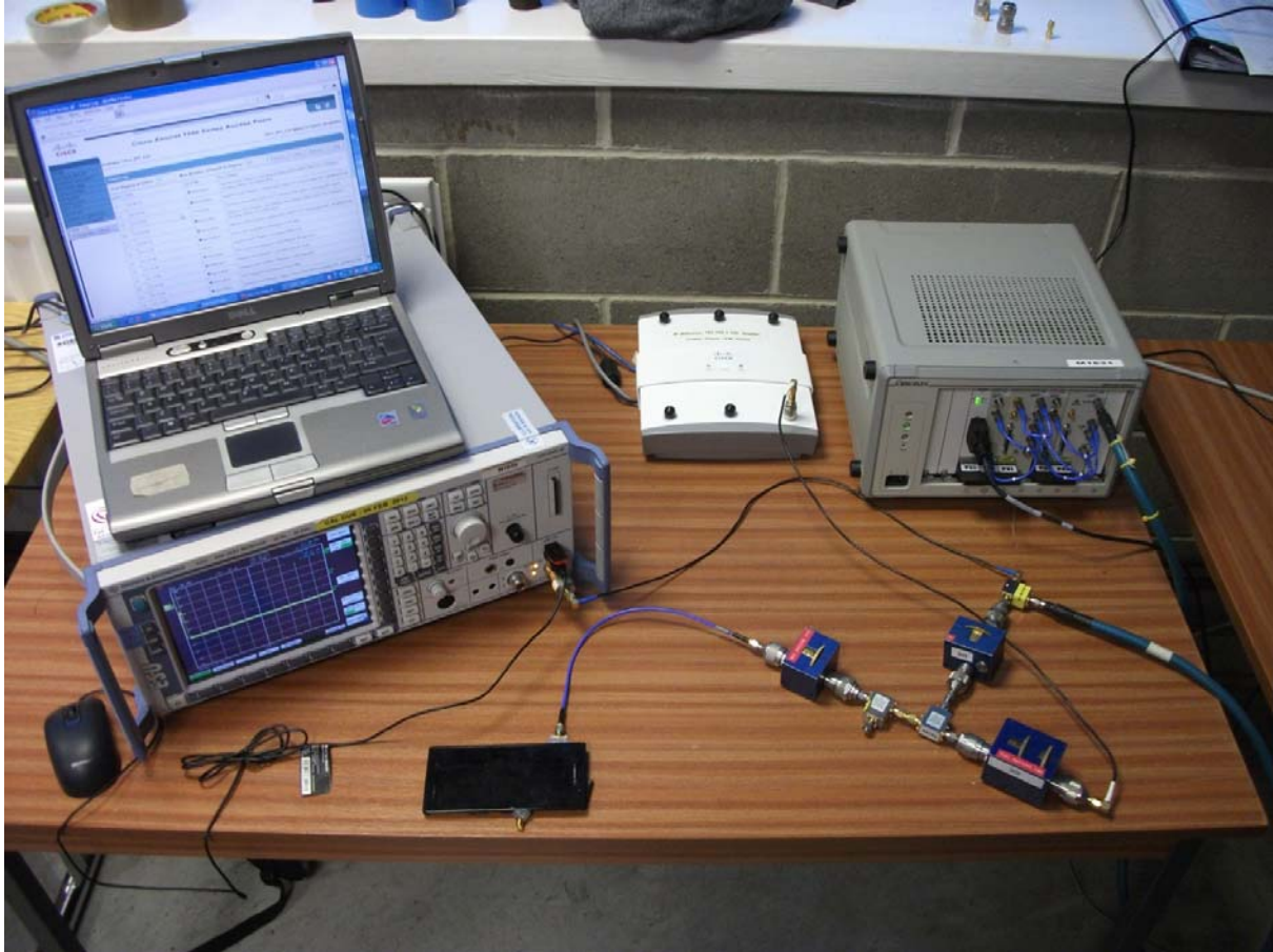
Test Set-up Overview
