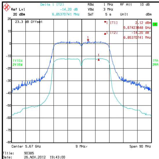
Top Channel / 5.47-5.725 GHz band
