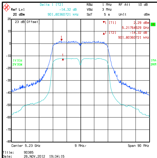
Top Channel / 5.15-5.25 GHz band
