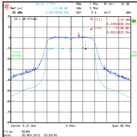
Top Channel / 5.25-5.35 GHz band
