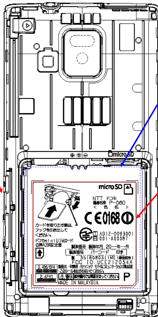
(Rear View)
