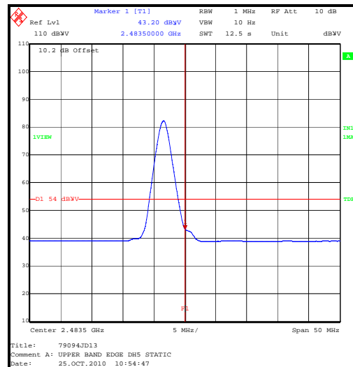
Upper Band Edge Average Static
