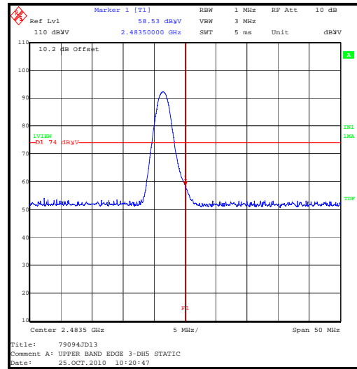
Upper Band Edge Peak Static
