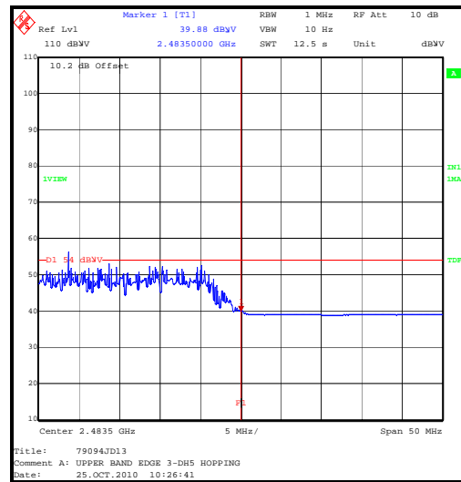
Upper Band Edge Average Hopping
