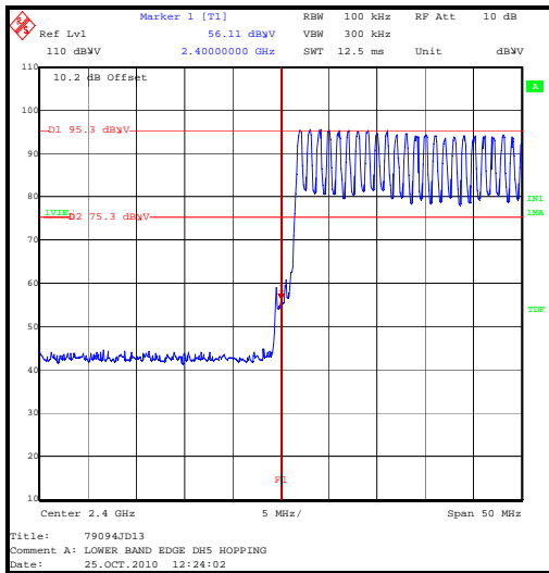
Lower Band Edge Peak Hopping
