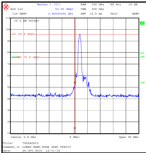
Lower Band Edge Peak Static
