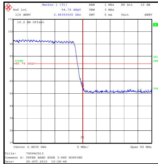
Upper Band Edge Peak Hopping
