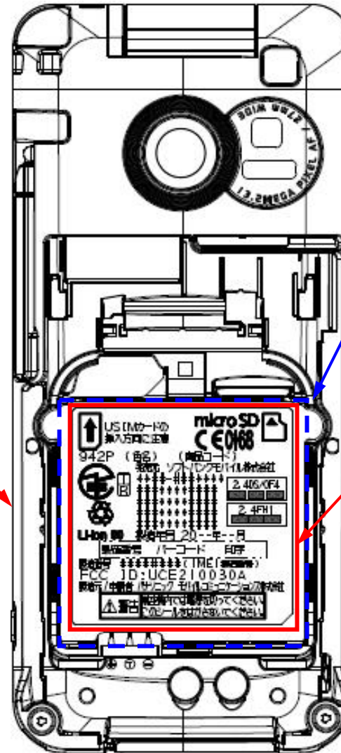
Label location
