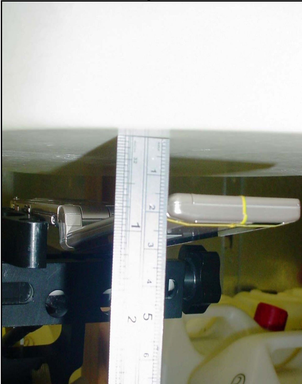
PHT/76421JD03/014: Front of EUT Facing Phantom With Antenna Retracted
