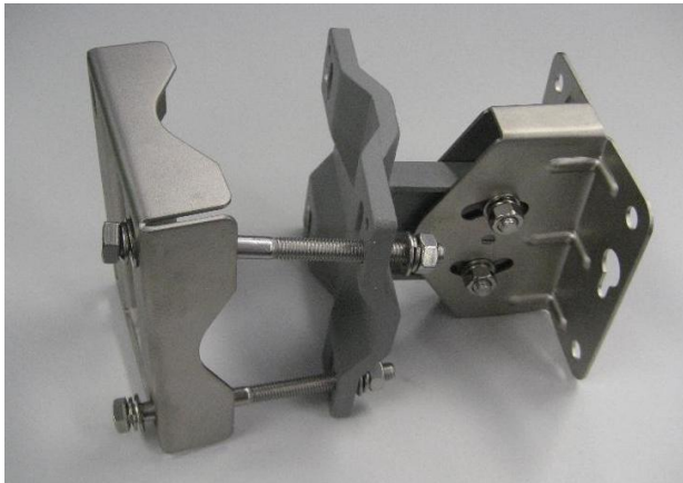
Figure 4. Mounting kit assembly
