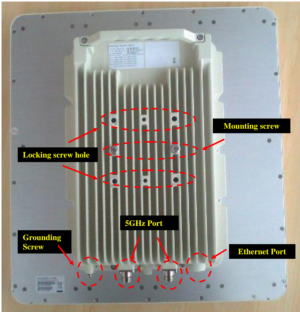
Figure 1. back-view of A8-Ein
