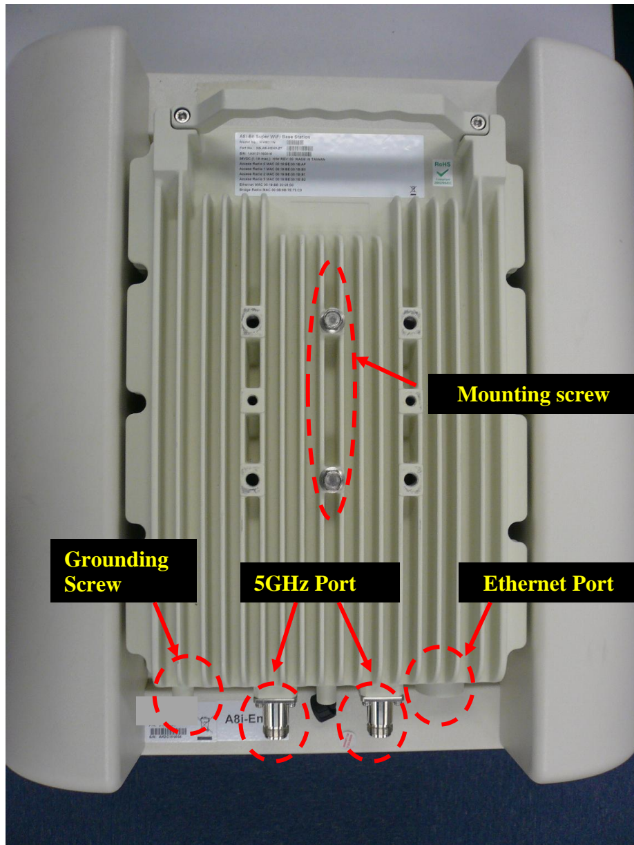
Figure 10. back-view of A8in
