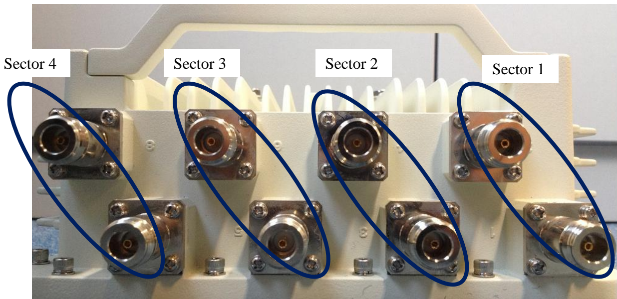
Figure21. A8n 2.4GHz RF port groups
