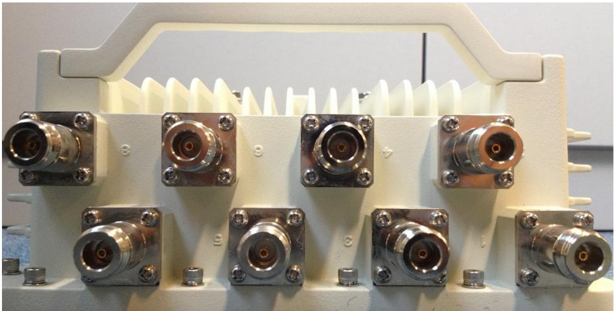
Figure16. Top of A8n – 8 N-female RF port for external 2.4GHz panel antenna connection
