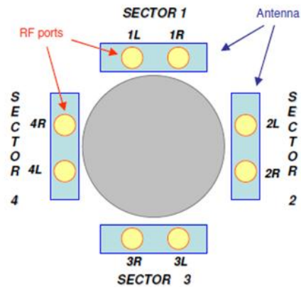
Figure 20. Antenna port to A8n port mapping
