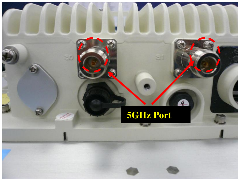
Figure 22. 5GHz “a0 & a1” antenna RF ports
