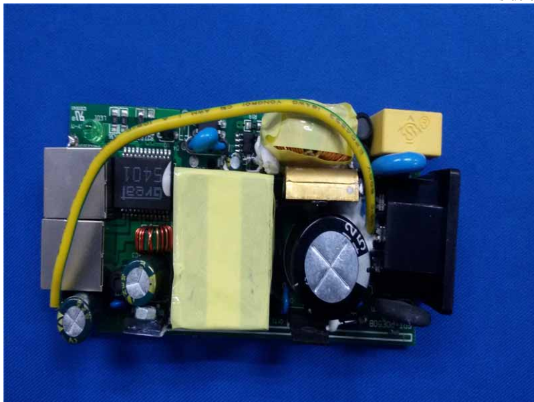
Figure 23 Inside of the Adapter
