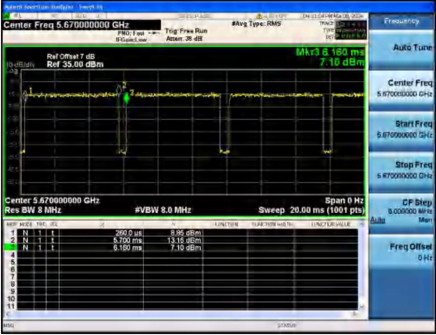
Duty Cycle_NVNT_ANT1_802_11ax(HE40)_5670
