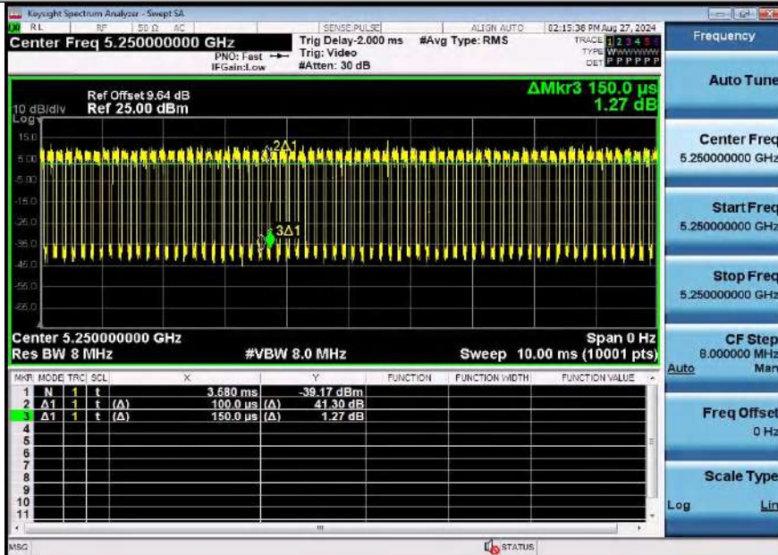
NTNV-11AX160SISO-Ant1-5250
