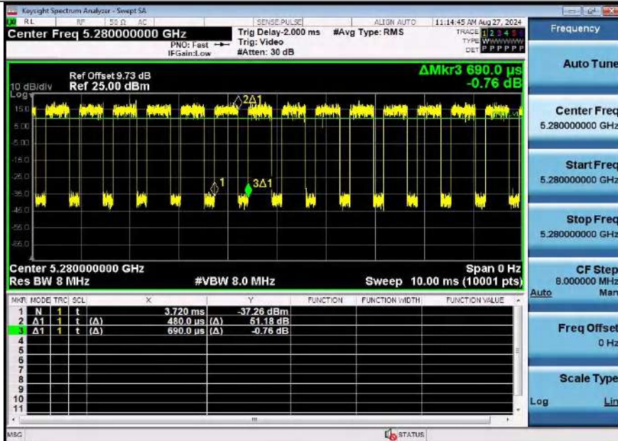
NTNV-11AX20SISO-Ant1-5280
