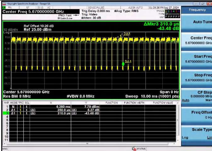
NTNV-11AX40SISO-Ant1-5670
