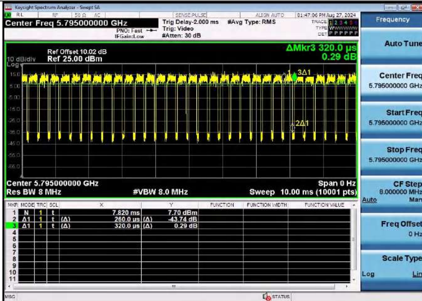
NTNV-11AX40SISO-Ant1-5795
