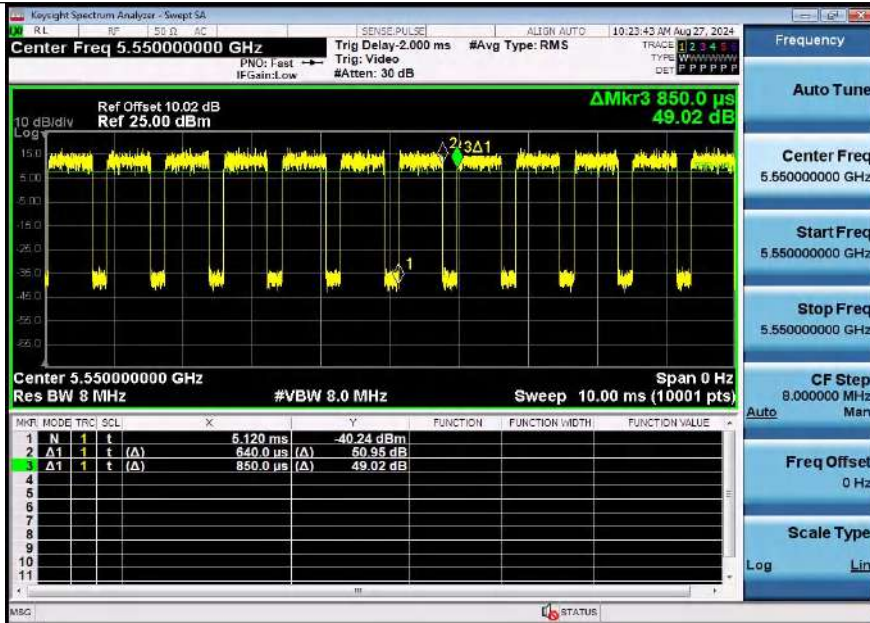
NTNV-11AC40SISO-Ant1-5550
