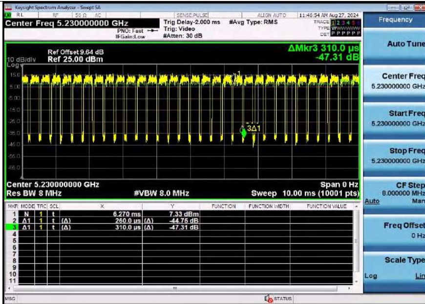
NTNV-11AX40SISO-Ant1-5230
