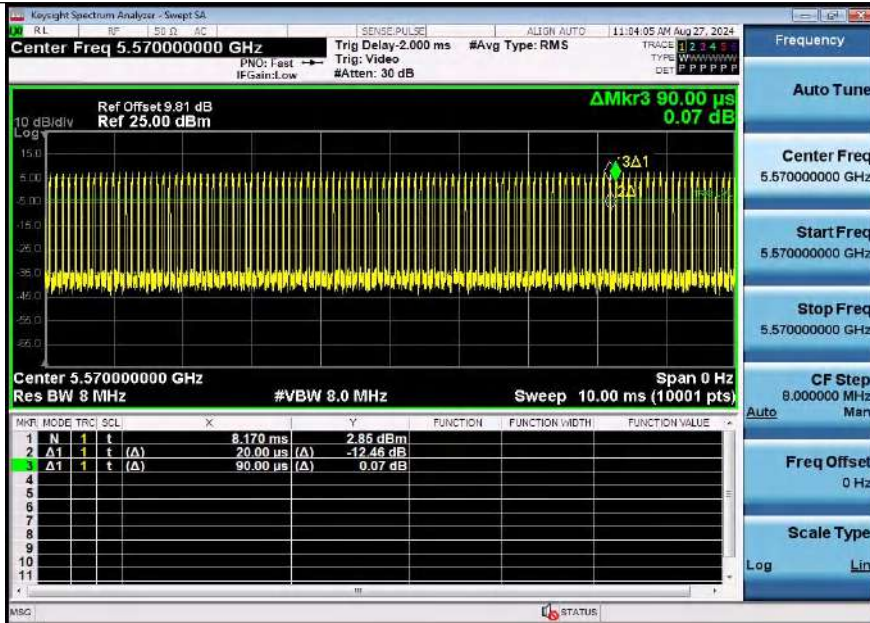
NTNV-11AC160SISO-Ant1-5570
