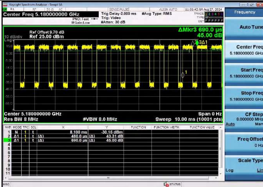
NTNV-11AX20SISO-Ant1-5180
