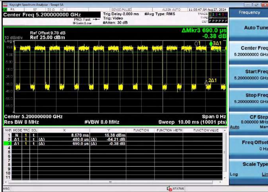
NTNV-11AX20SISO-Ant1-5200
