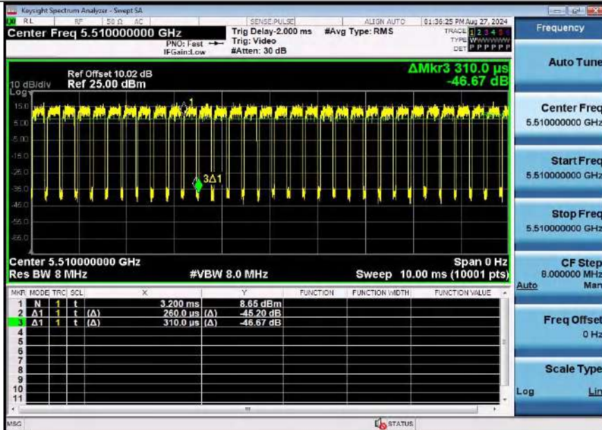
NTNV-11AX40SISO-Ant1-5510
