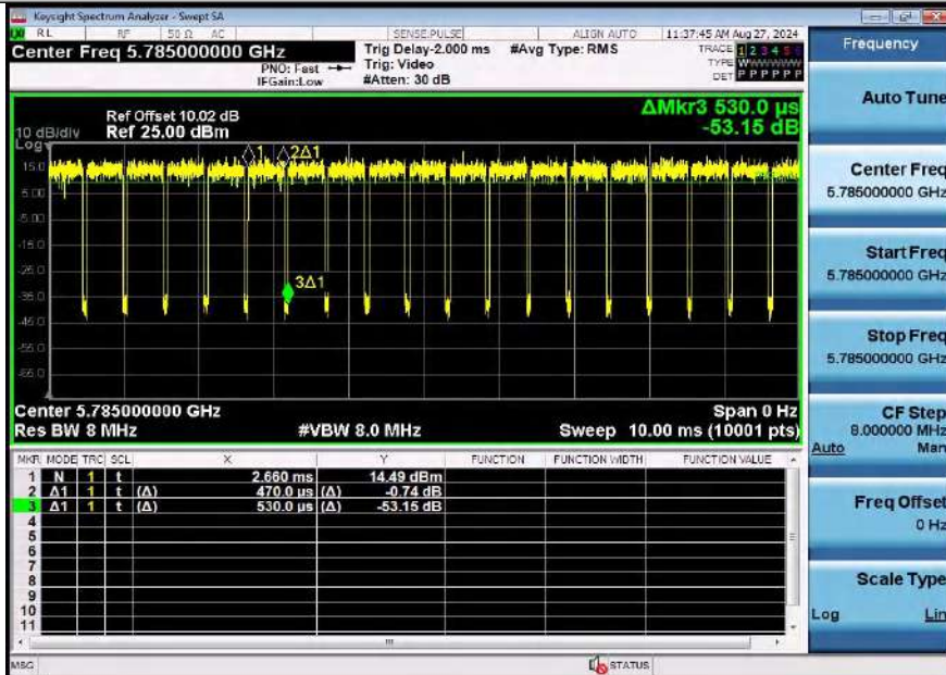
NTNV-11AX20SISO-Ant1-5785
