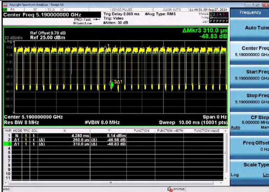
NTNV-11AX40SISO-Ant1-5190
