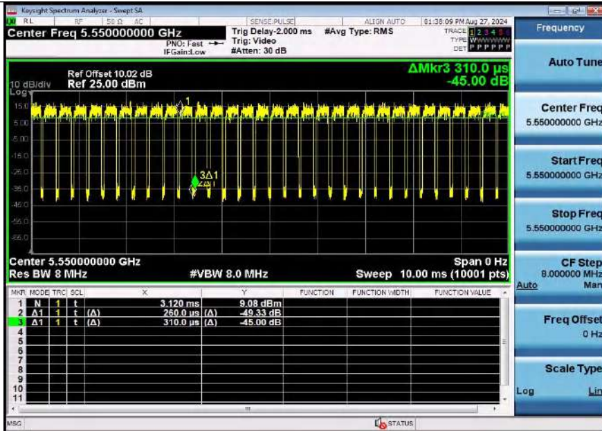
NTNV-11AX40SISO-Ant1-5550
