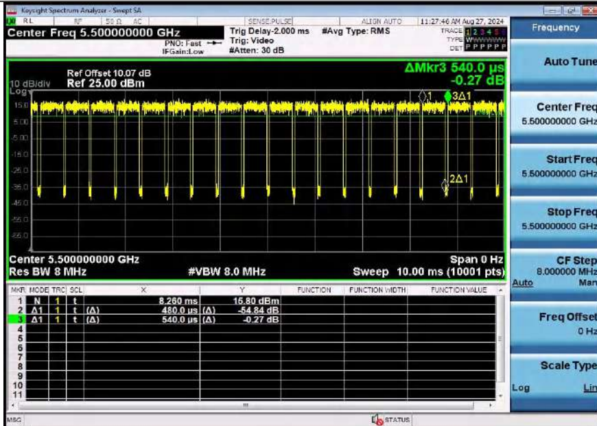
NTNV-11AX20SISO-Ant1-5500
