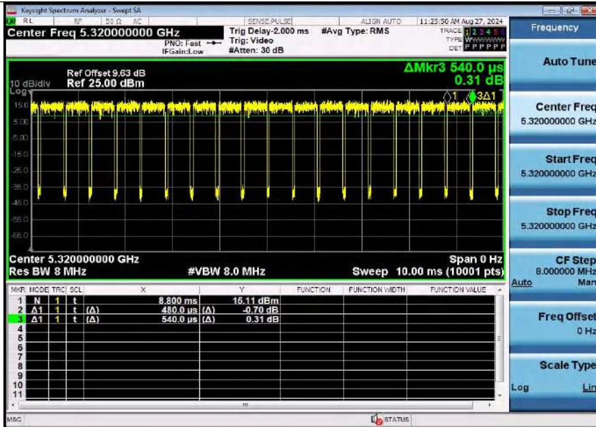
NTNV-11AX20SISO-Ant1-5320
