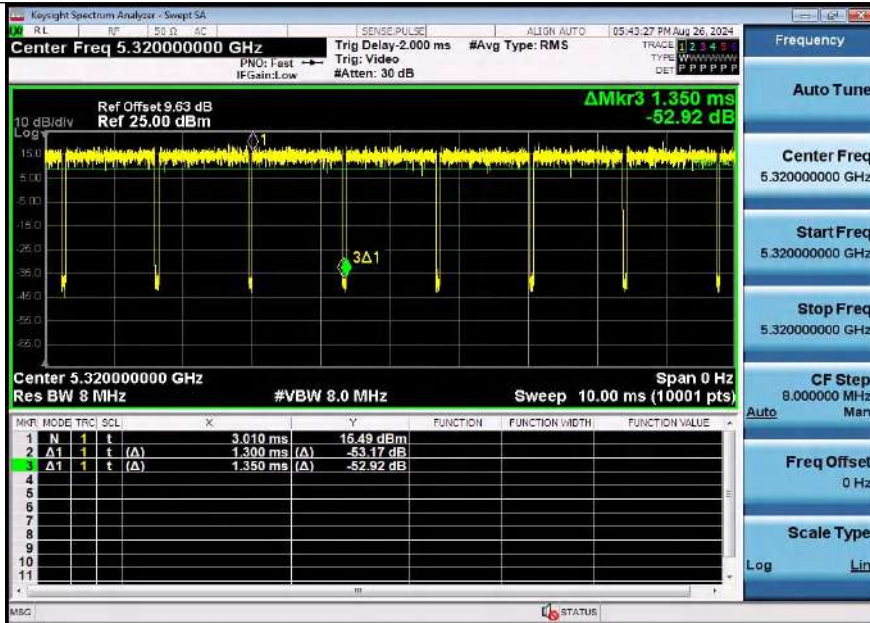
NTNV-11AC20SISO-Ant1-5320
