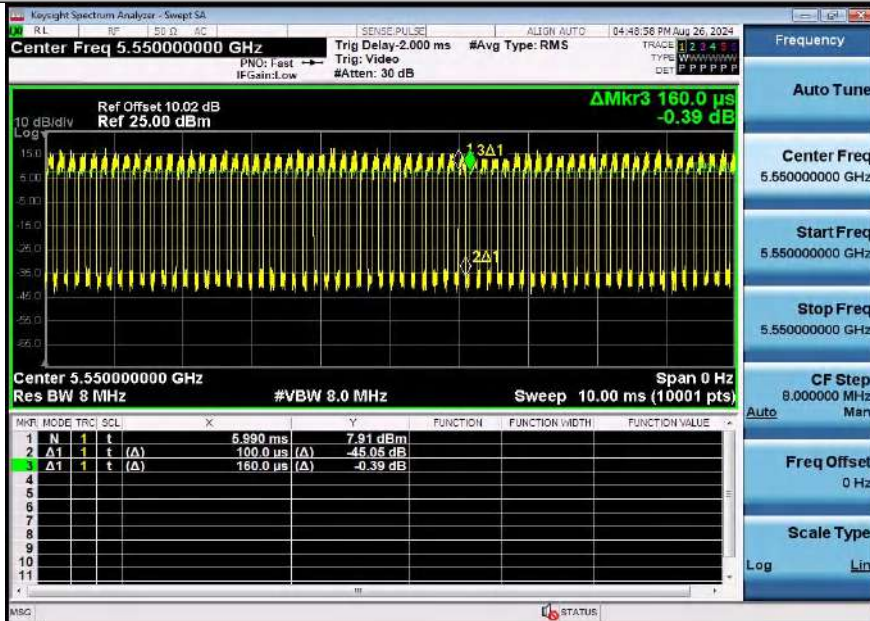
NTNV-11N40SISO-Ant1-5550
