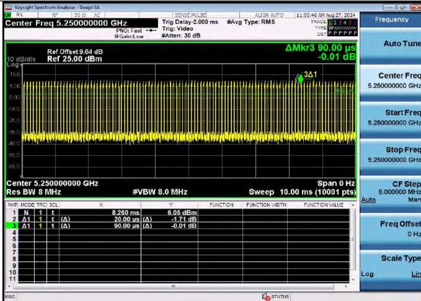
NTNV-11AC160SISO-Ant1-5250
