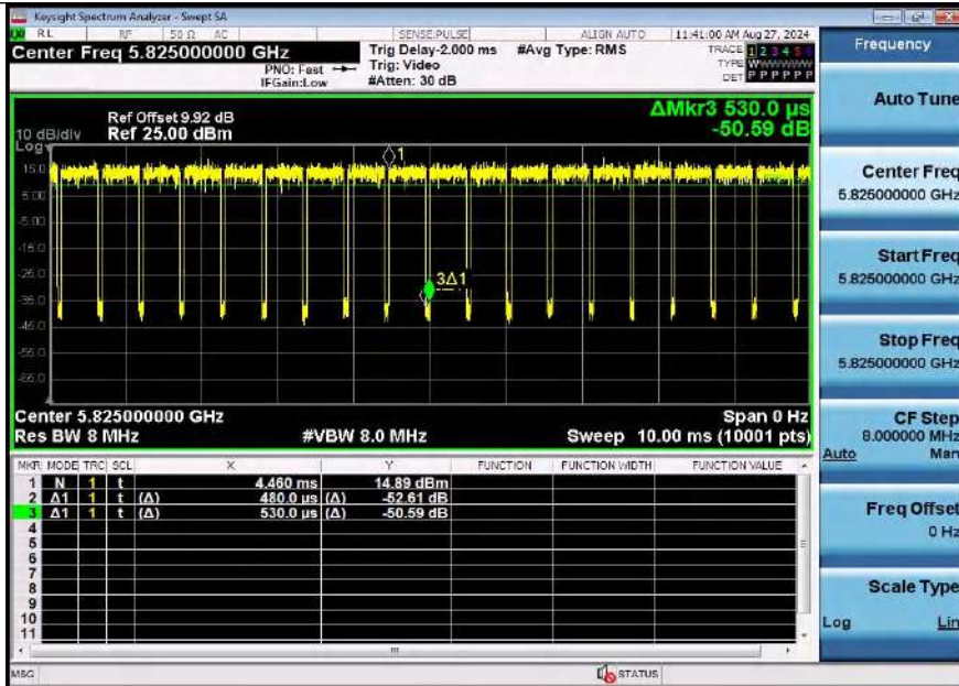
NTNV-11AX20SISO-Ant1-5825
