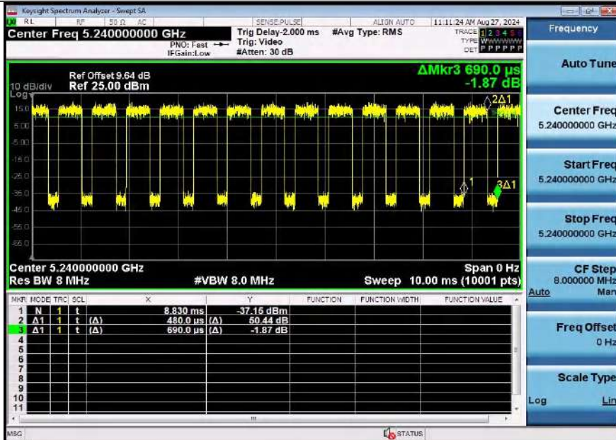
NTNV-11AX20SISO-Ant1-5240
