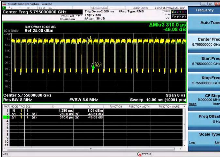
NTNV-11AX40SISO-Ant1-5755
