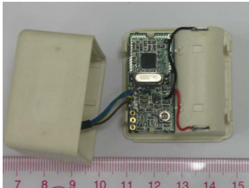
Transmitter
