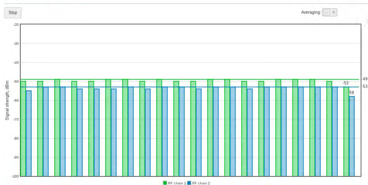
Figure 49 – Antenna Alignment
