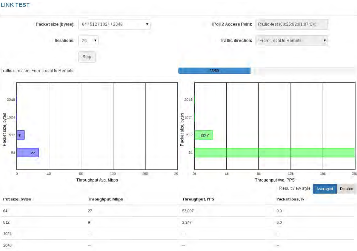
Figure 51 – Linktest Results
