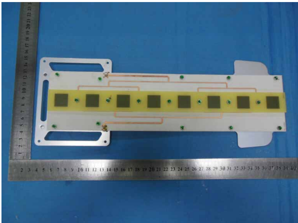
EUT-19dBi Antenna View
