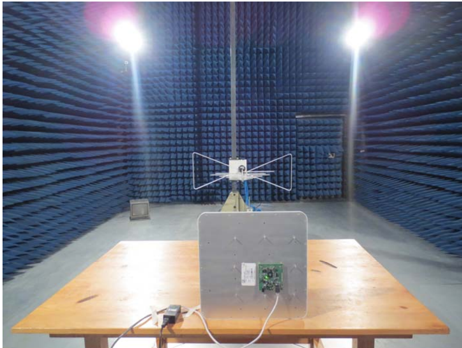
Radiated emission(23 dBi antenna)
