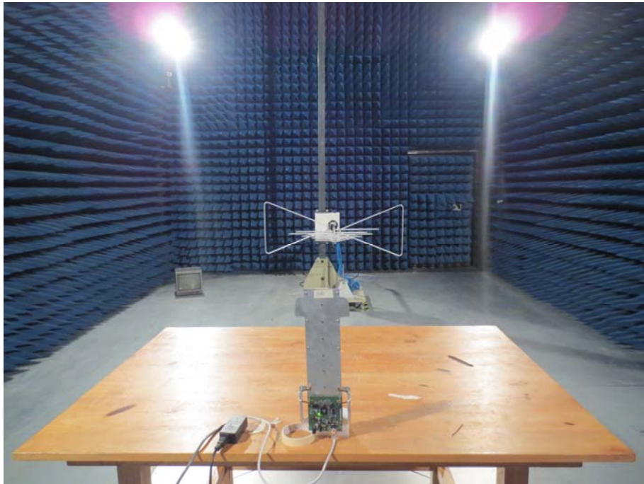
Radiated emission(19 dBi antenna)
