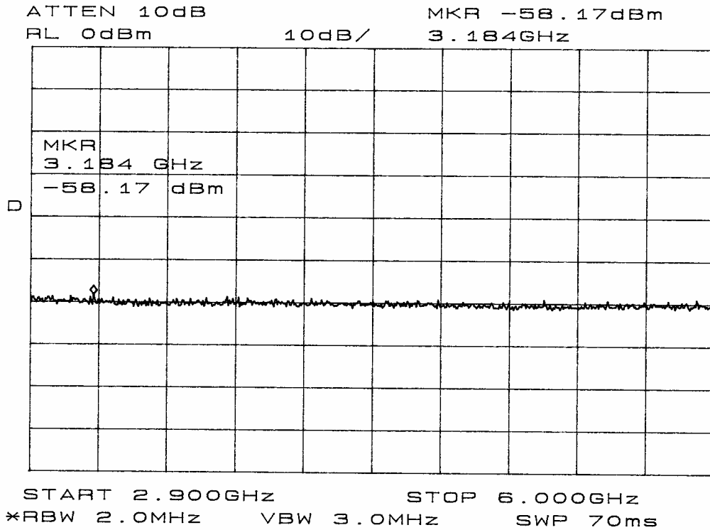
Figure 19 Antenna Emission plot taken in screen room.
