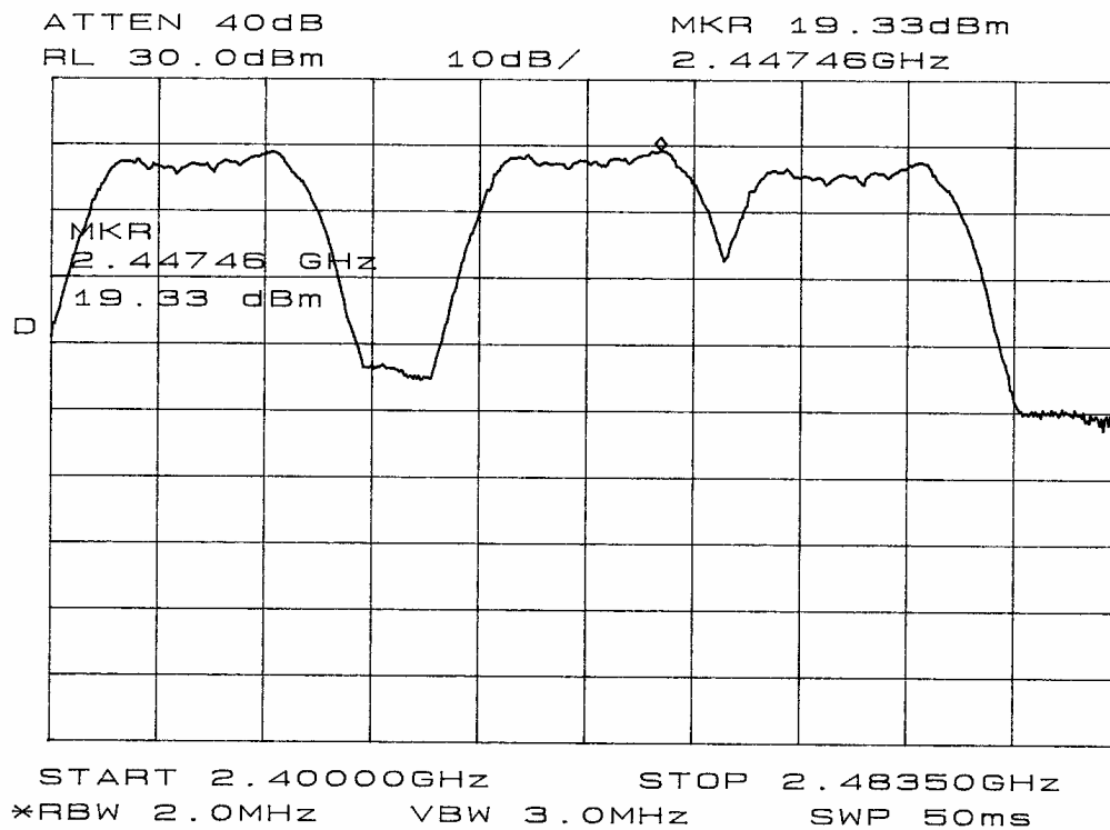
Figure 10 maximum power plot taken in screen room (Mode G).
