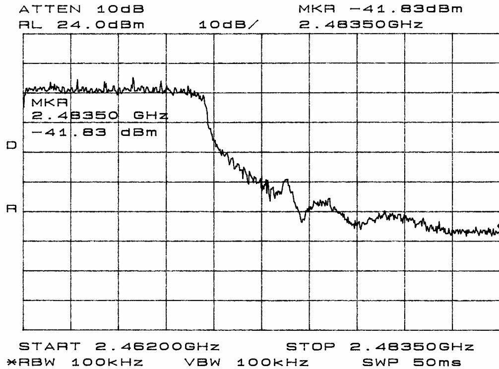
Figure 31 Antenna Conducted Band Edge plot taken in screen room (Mode G).
