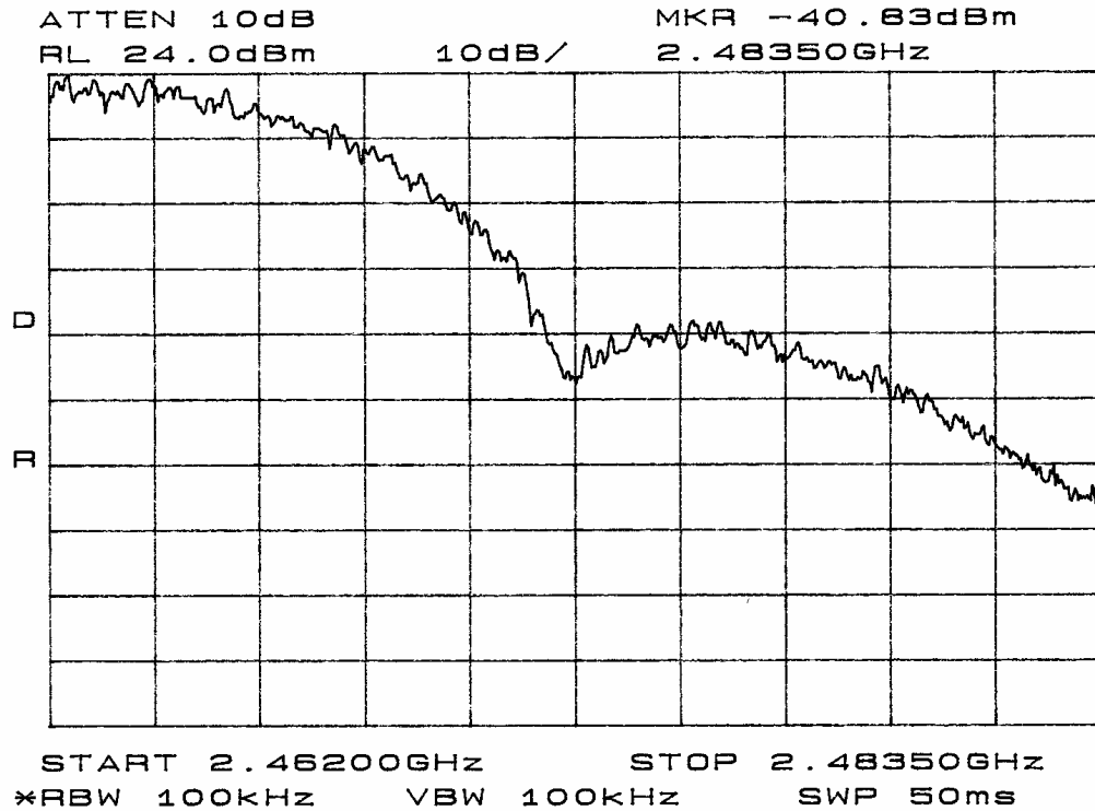
Figure 29 Antenna Conducted Band Edge plot taken in screen room (Mode B).
