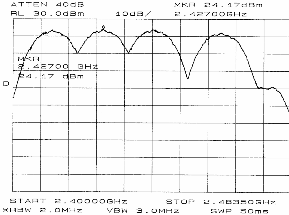
Figure 9 maximum power plot taken in screen room (Mode B).
