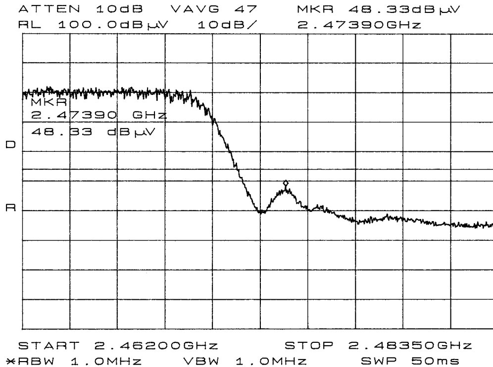
Figure 35 3-meter Radiated Emission Band Edge plot (Mode G).
