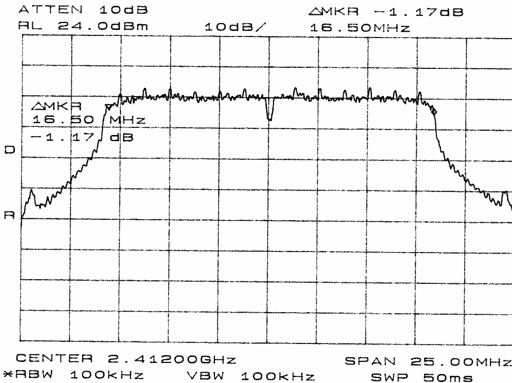
Figure 14 6dB Band width Requirement plot taken in screen room (Mode G).
