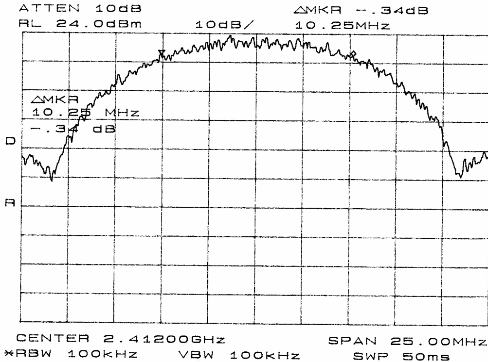
Figure 11 6dB Band width Requirement plot taken in screen room (Mode B).
