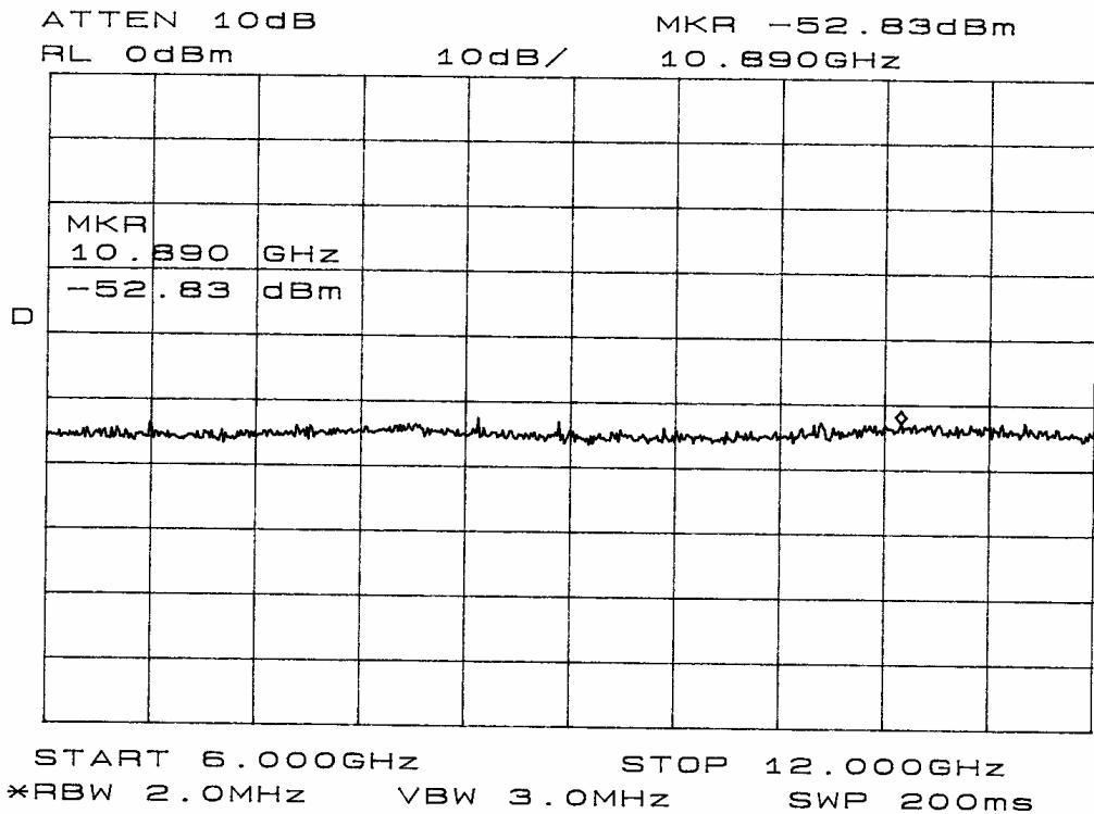
Figure 20 Antenna Emission plot taken in screen room.
