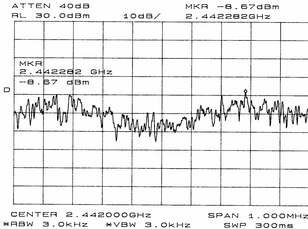
Figure 26 Power Spectral Density plot taken in screen room (Mode G).
