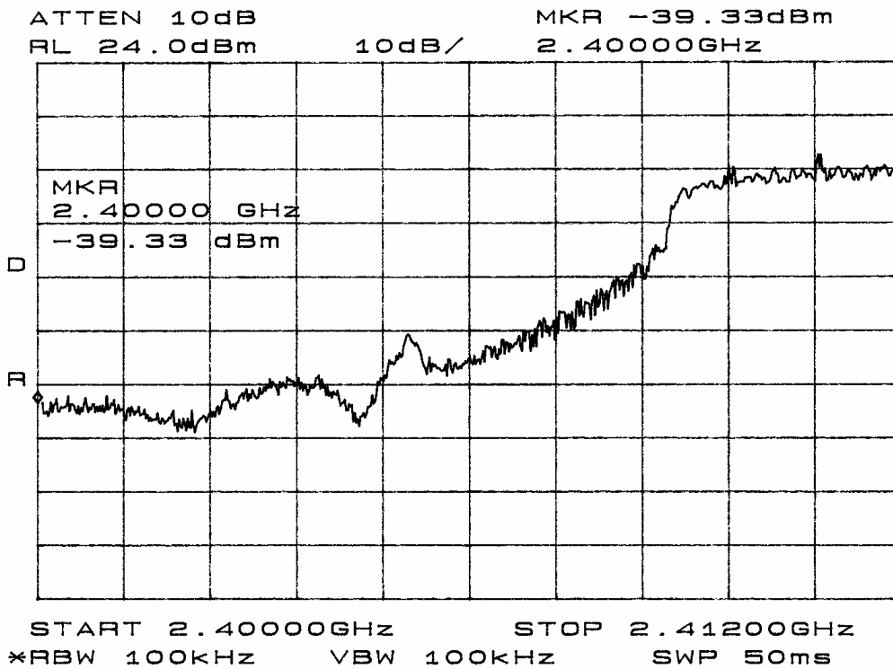
Figure 30 Antenna Conducted Band Edge plot taken in screen room (Mode G).
