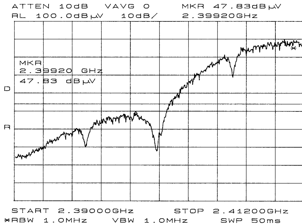
Figure 32 3-meter Radiated Emission Band Edge plot (Mode B).
