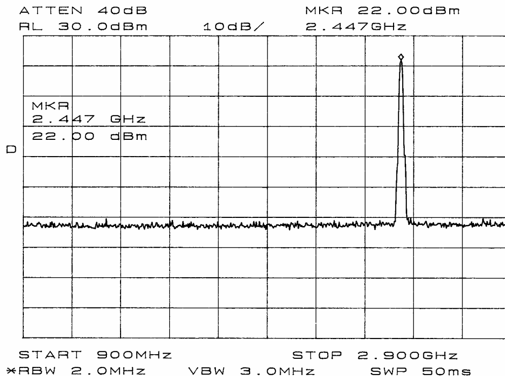
Figure 18 Antenna Emission plot taken in screen room.
