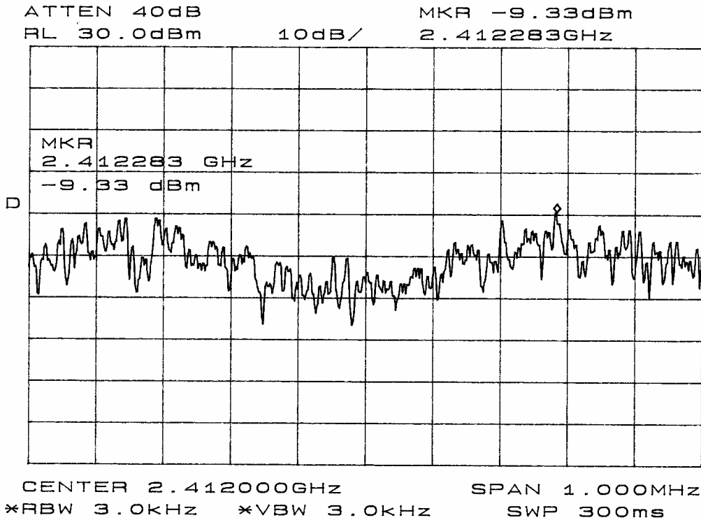
Figure 25 Power Spectral Density plot taken in screen room (Mode G).
