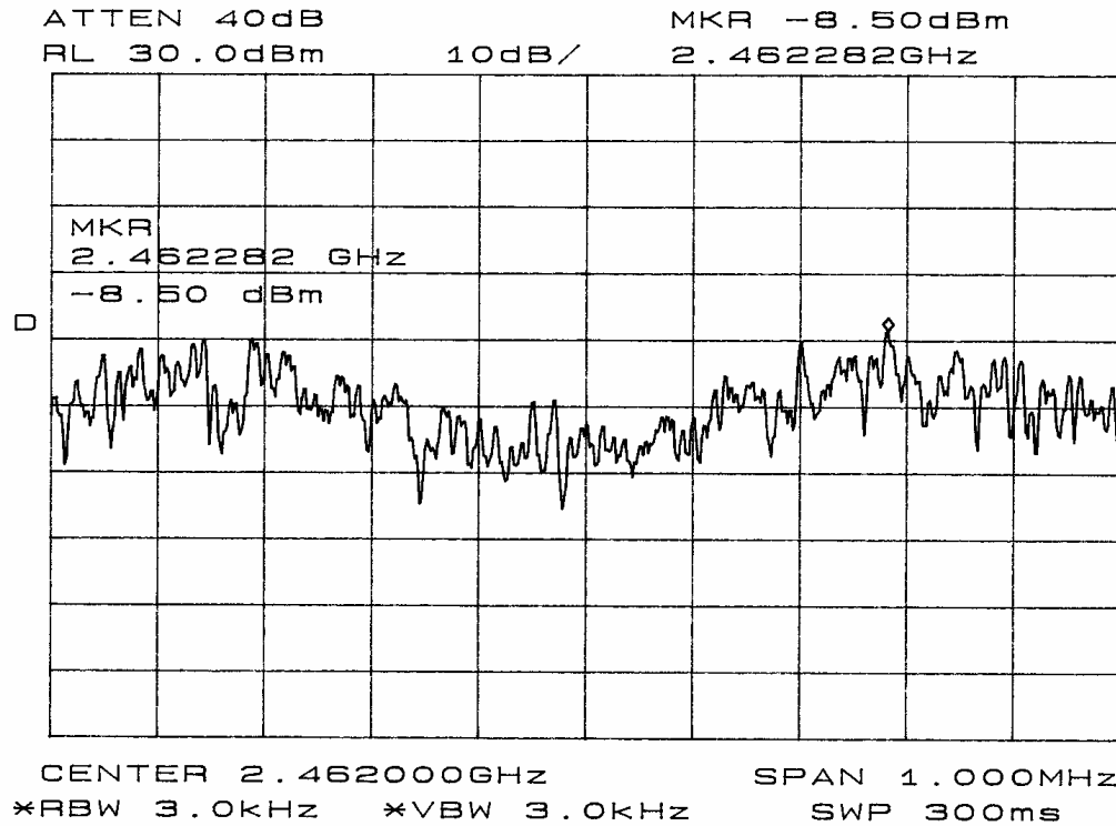
Figure 27 Power Spectral Density plot taken in screen room (Mode G).
