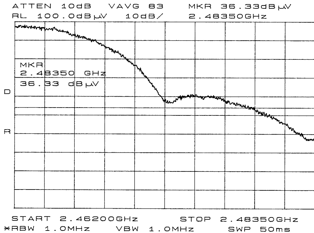
Figure 33 3-meter Radiated Emission Band Edge plot (Mode B).
