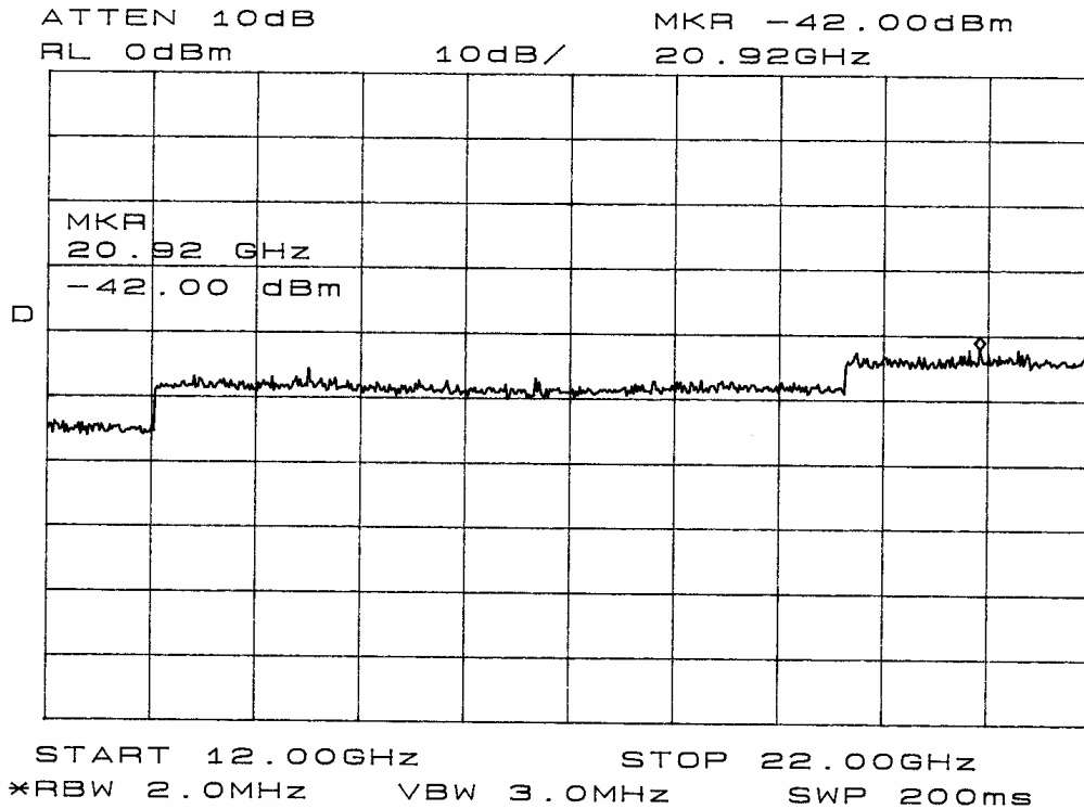
Figure 21 Antenna Emission plot taken in screen room.
