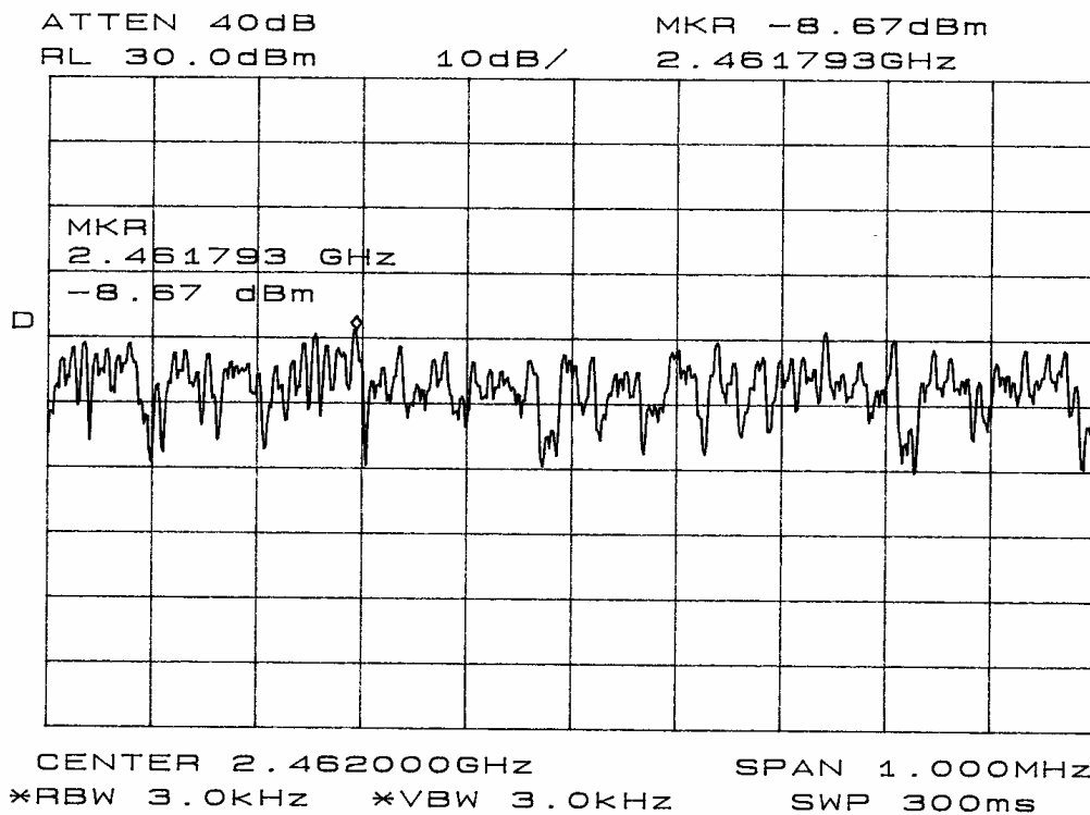
Figure 24 Power Spectral Density plot taken in screen room (Mode B).
