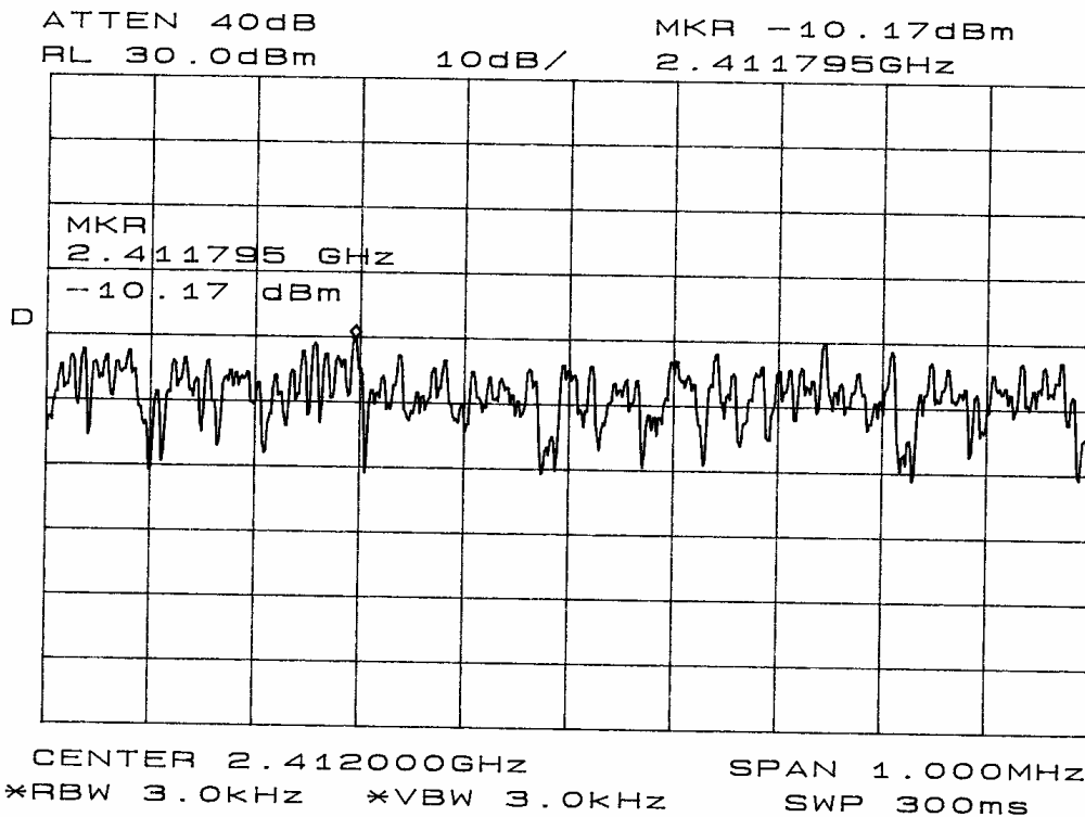
Figure 22 Power Spectral Density plot taken in screen room (Mode B).
