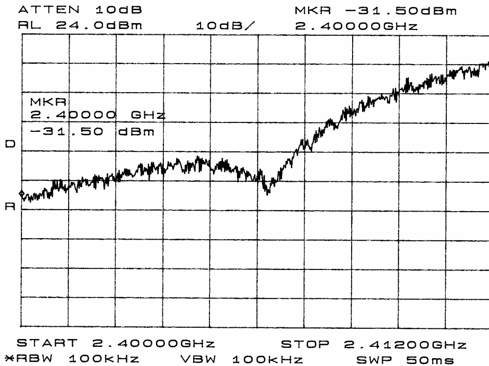
Figure 28 Antenna Conducted Band Edge plot taken in screen room (Mode B).
