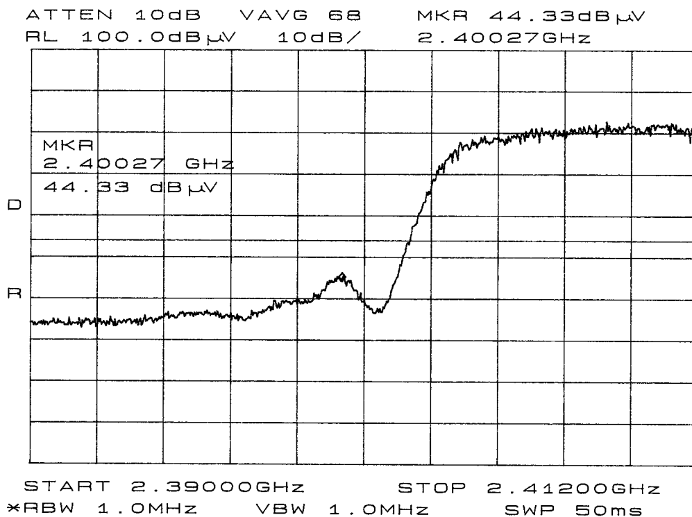
Figure 34 3-meter Radiated Emission Band Edge plot (Mode G).
