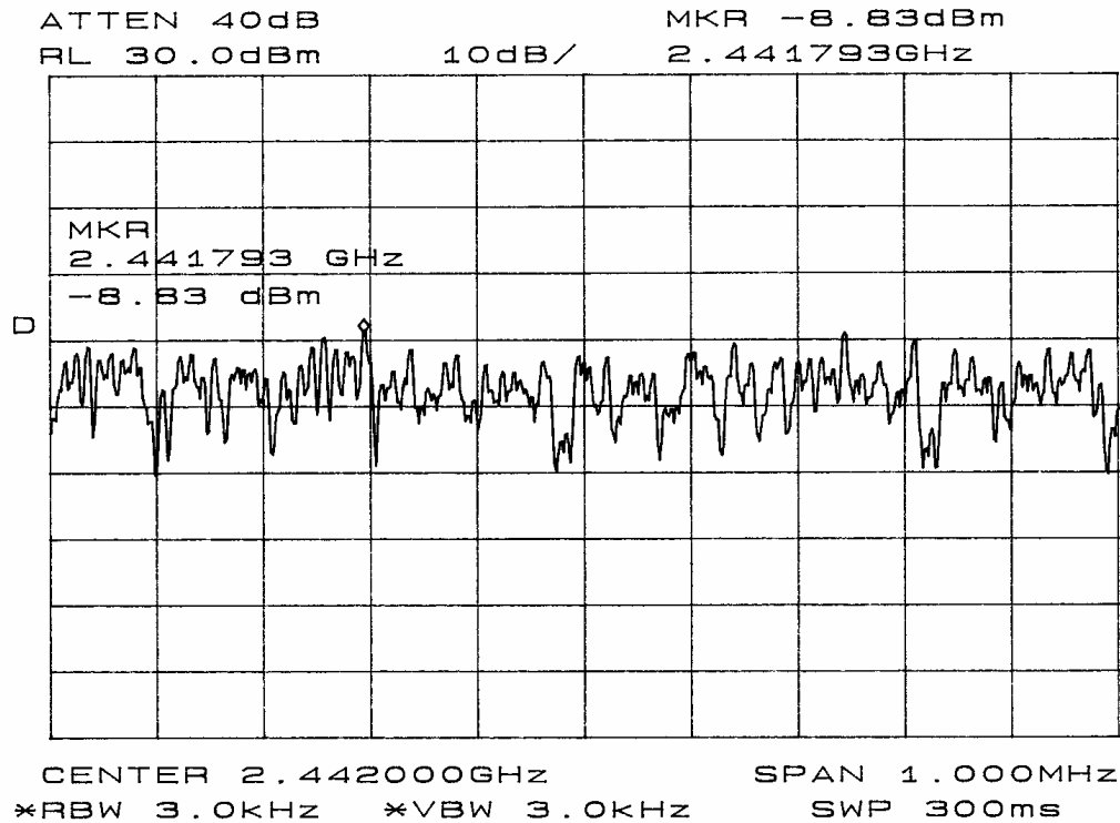
Figure 23 Power Spectral Density plot taken in screen room (Mode B).
