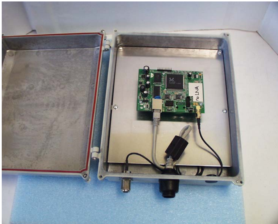
Printed circuit board mounted inside DLB2100 enclosure.
