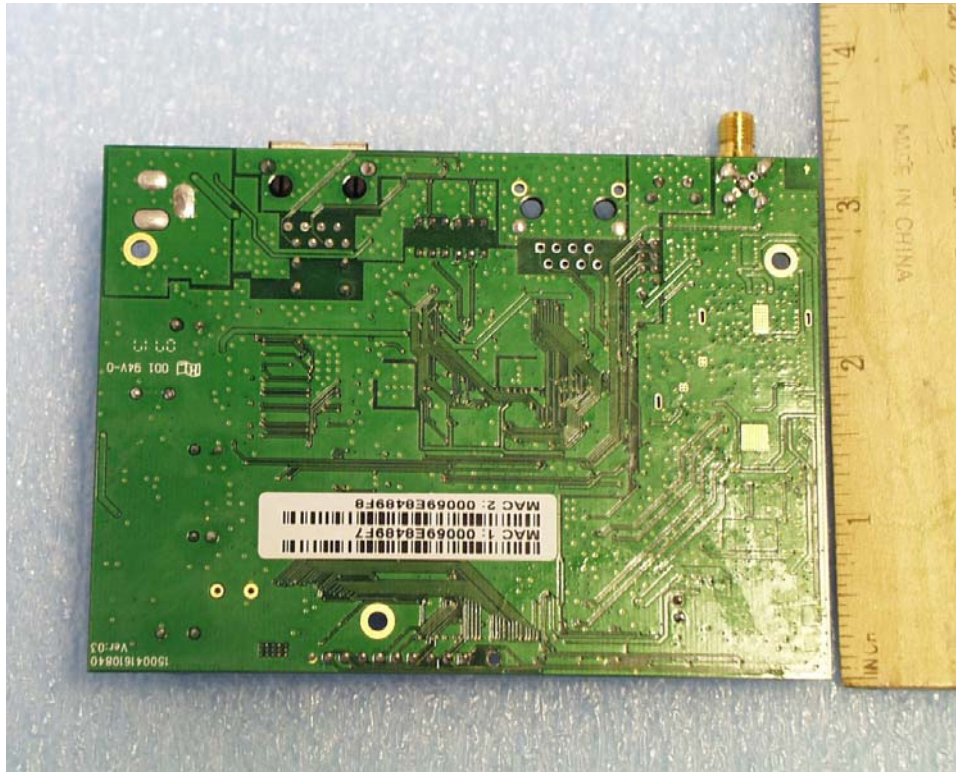
Solder side of printed circuit board
