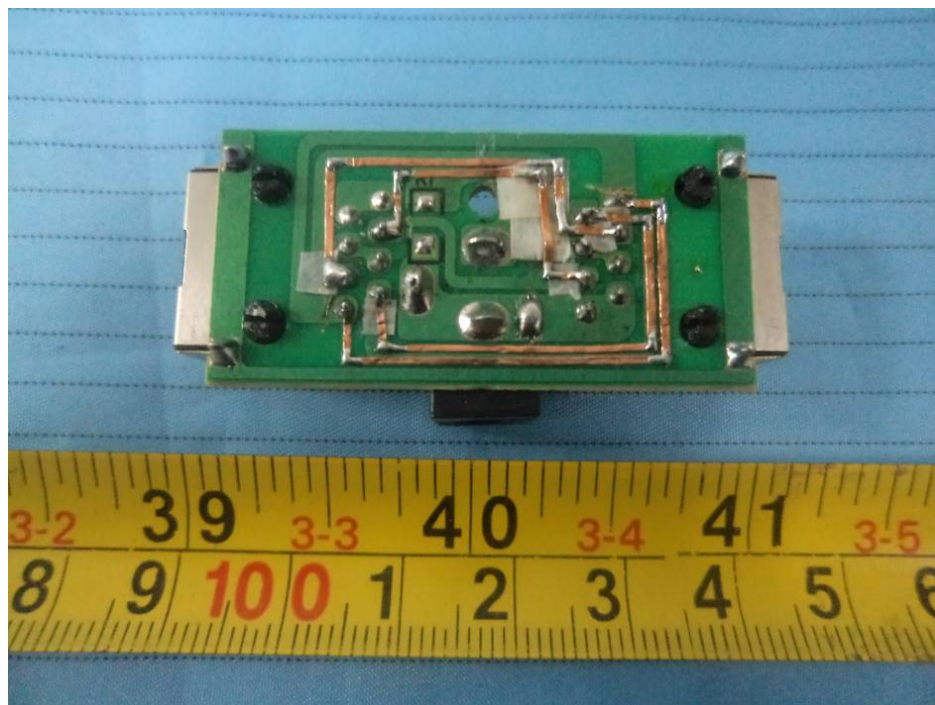
EUT – PoE Board Bottom View
