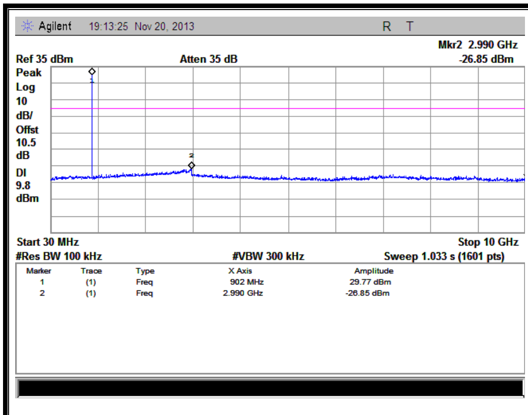
(Plot D.1: Channel = 1, 30MHz to 10GHz @ Profile 2)
