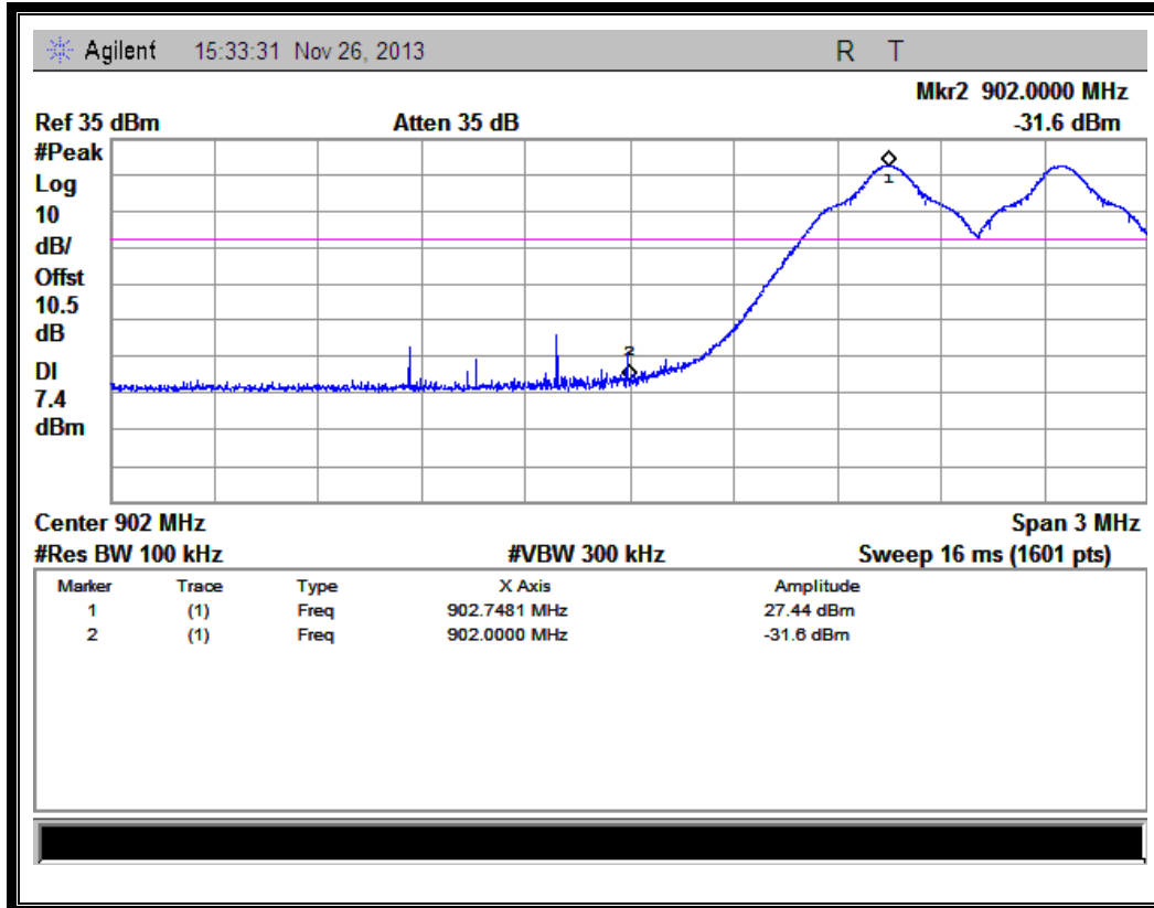
(Channel = 1, Band edge with hopping on @ Profile 4)
