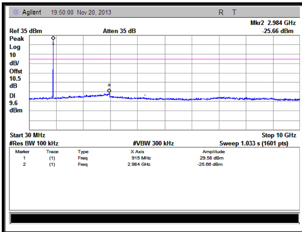
(Plot B.1: Channel = 26, 30MHz to 10GHz @ Profile 1)
