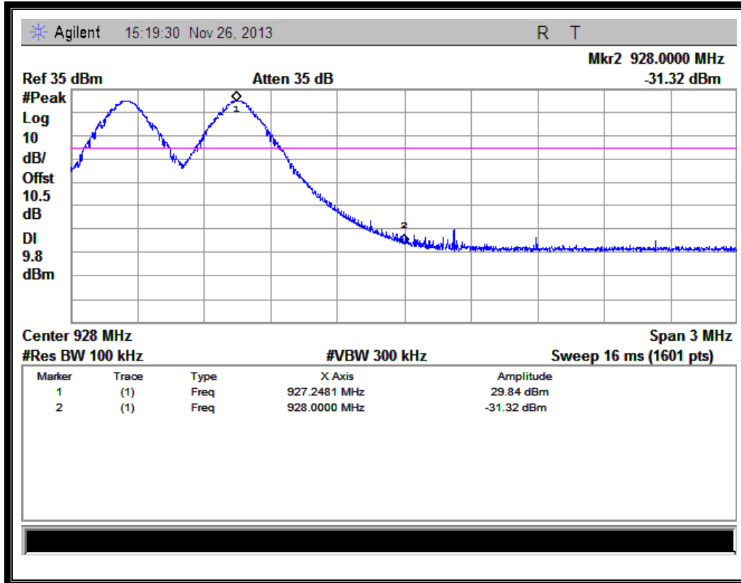
(Channel = 50, Band edge with hopping on @ Profile 1)
