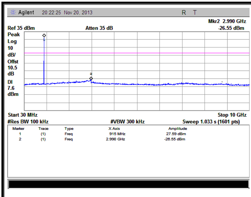
(Plot H.1: Channel = 26, 30MHz to 10GHz @ Profile 4)
