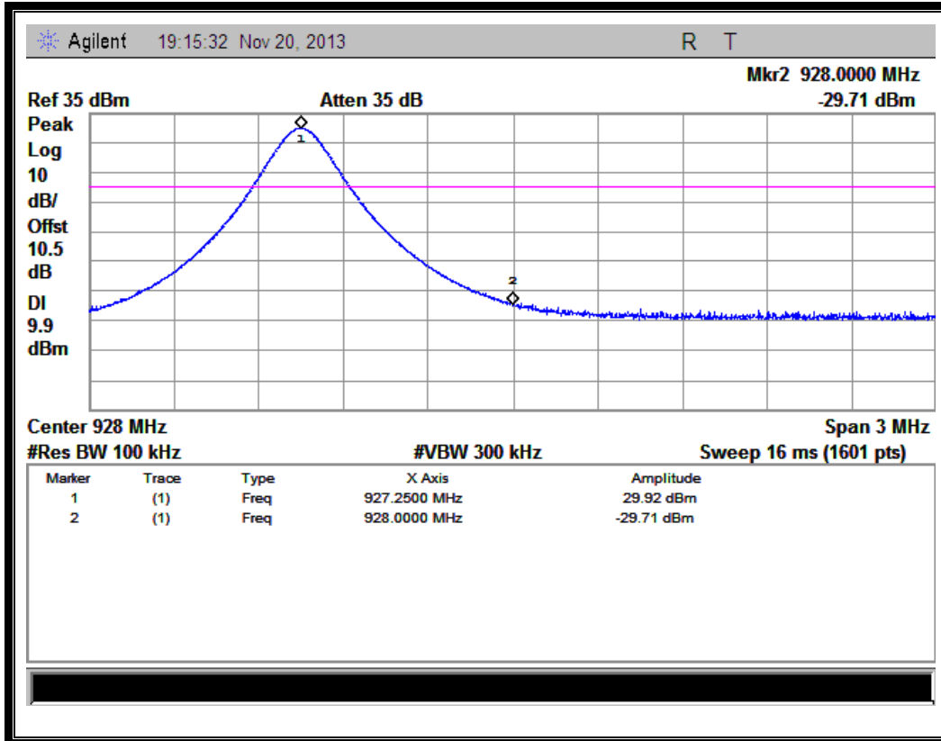
(Channel = 50, Band edge @ Profile 2)
