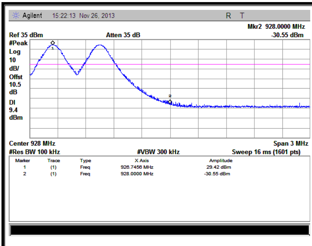
(Channel = 50, Band edge with hopping on @ Profile 2)
