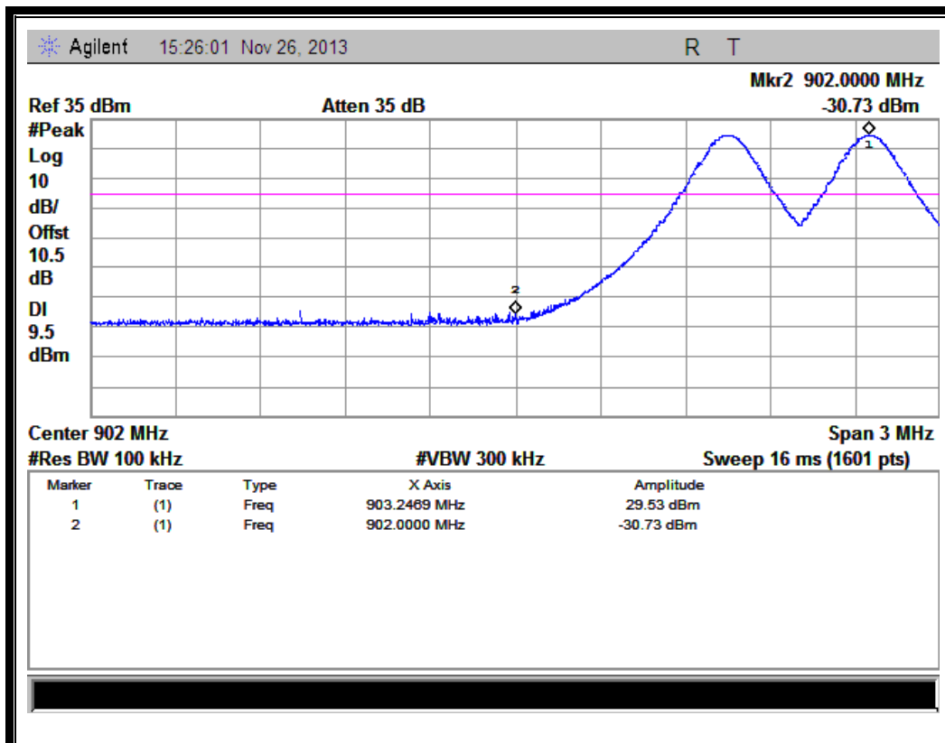
(Channel = 1, Band edge with hopping on @ Profile 2)
