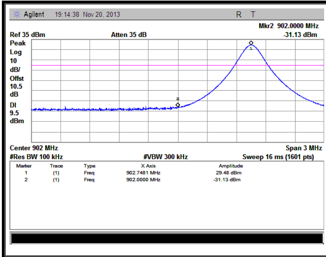
(Channel = 1, Band edge @ Profile 2)
