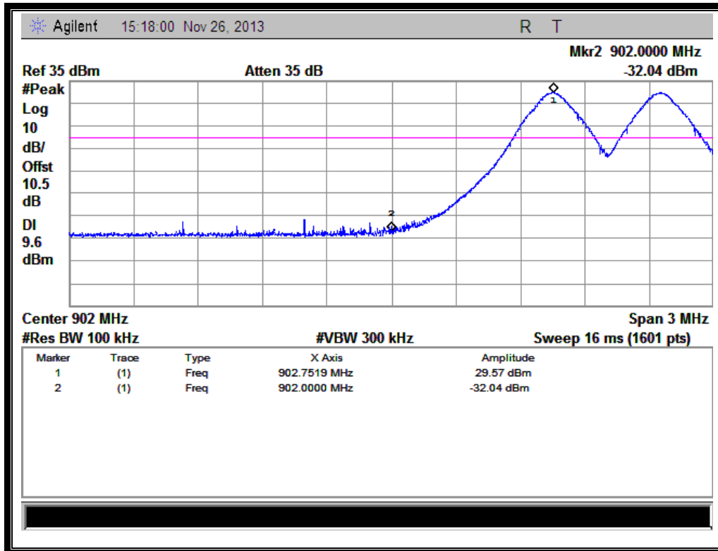
(Channel = 1, Band edge with hopping on Profile 1)
