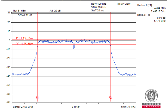
802.11n (HT20): Chain 1 / CH10
