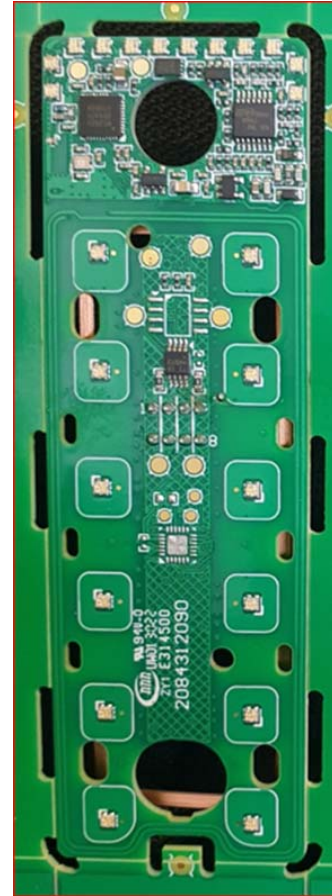
Bottom Side of Unpotted PCB
