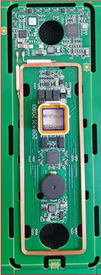
Top Side of Unpotted PCB
