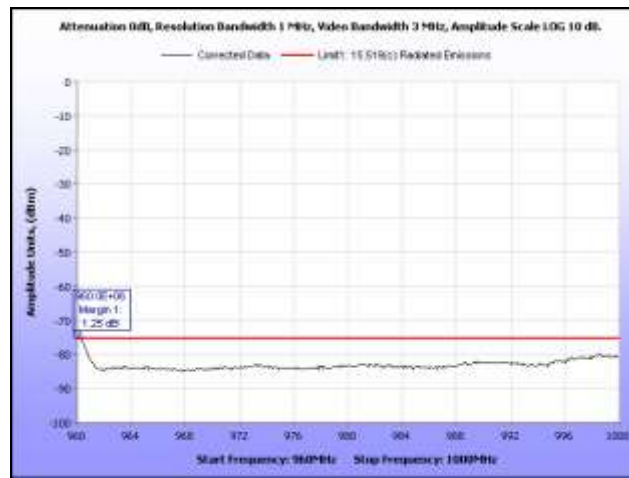
Plot 24. Radiated Emissions, 960 MHz – 1 GHz, BG3
