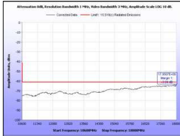
Plot 29. Radiated Emissions, 10.6 GHz – 18 GHz, BG3
