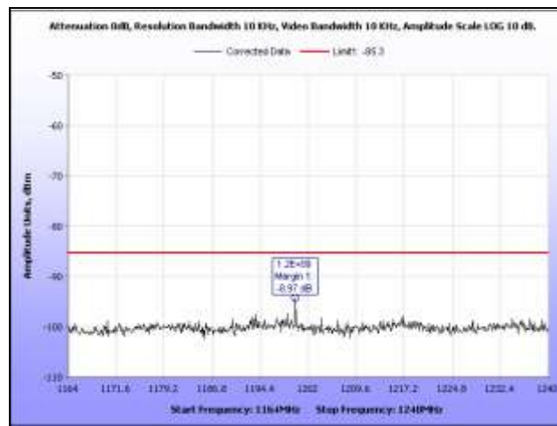
Plot 43. Radiated Emissions, 1.164 GHz – 1.24 GHz, GPS Band, BG6
