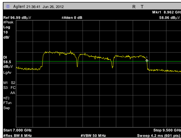
Plot 14. UWB Bandwidth, F_h , BG6
