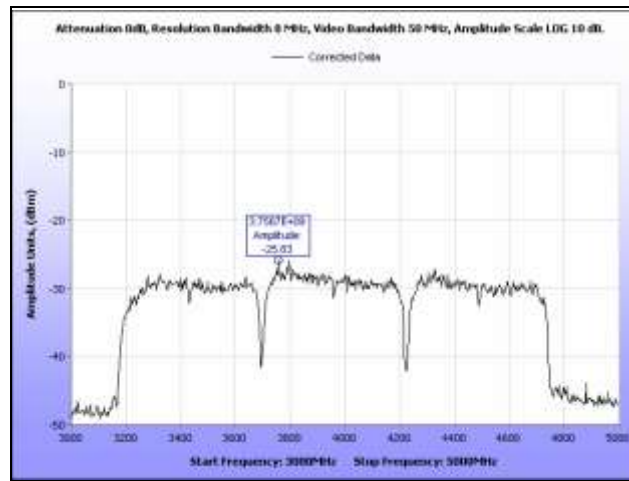
Plot 45. Peak Emissions, Field Strength, BG1
