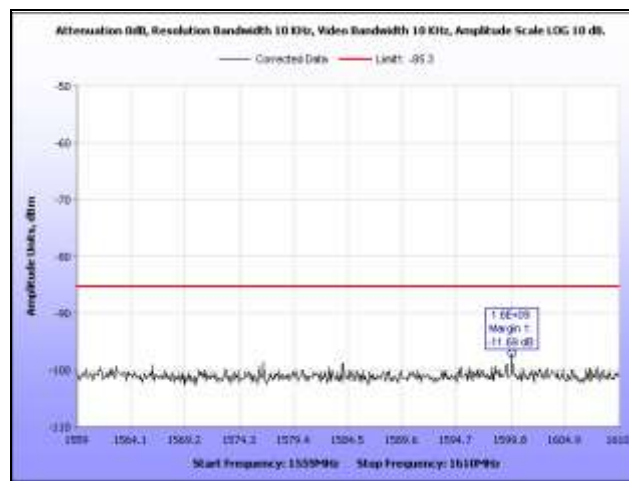
Plot 44. Radiated Emissions, 1.559 GHz – 1.61 GHz, GPS Band, BG6
