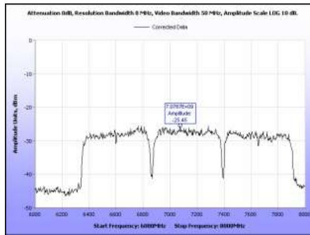
Plot 46. Peak Emissions, Field Strength, BG3
