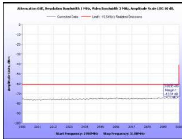
Plot 27. Radiated Emissions, 1.99 GHz – 3.1 GHz, BG3
