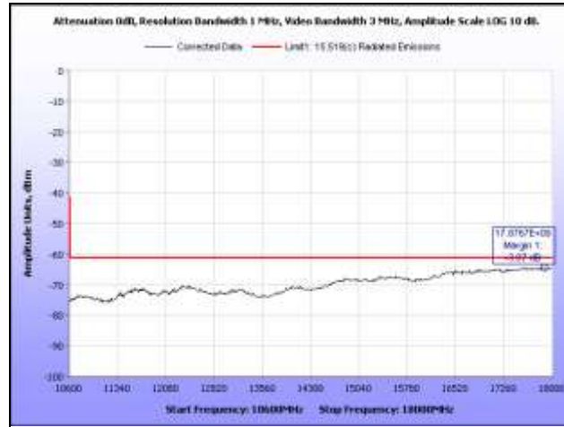
Plot 37. Radiated Emissions, 10.6 GHz – 18 GHz, BG6
