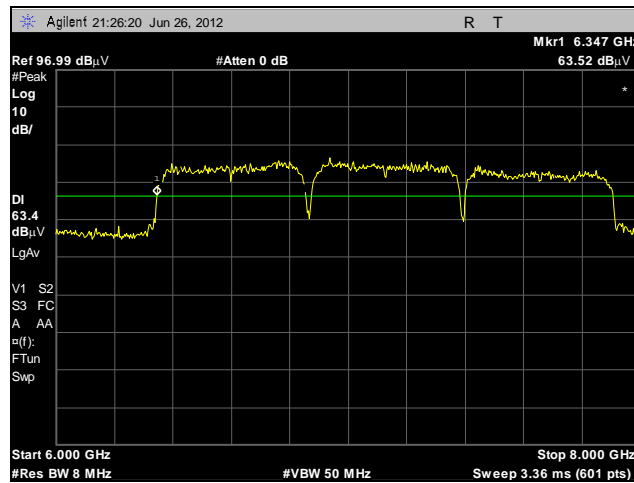
Plot 10. UWB Bandwidth, F_l , BG3
