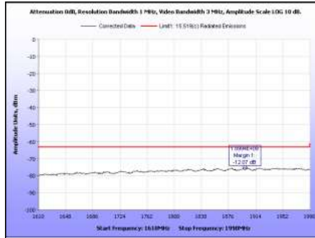
Plot 18. Radiated Emissions, 1.61 GHz – 1.99 GHz, BG1
