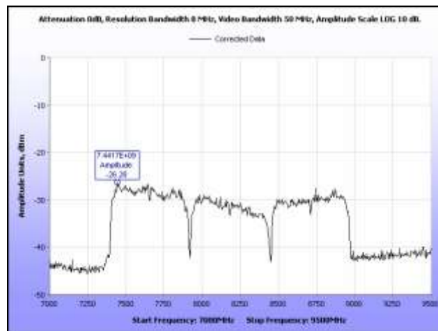
Plot 47. Peak Emissions, Field Strength, BG6
