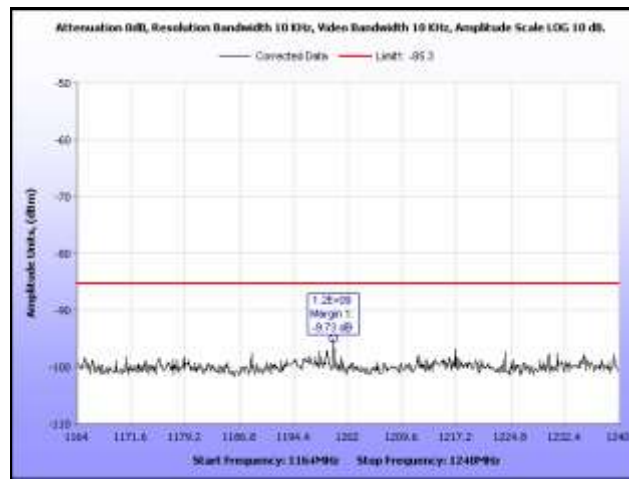
Plot 39. Radiated Emissions, 1.164 GHz – 1.24 GHz, GPS Band, BG1
