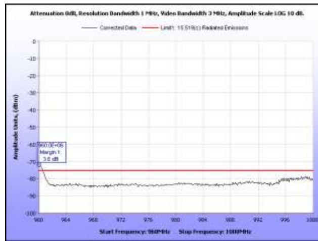
Plot 32. Radiated Emissions, 960 MHz – 1 GHz, BG6
