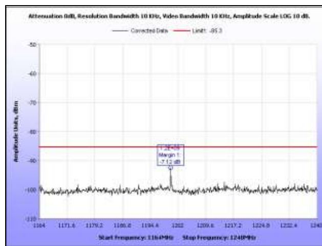
Plot 41. Radiated Emissions, 1.164 GHz – 1.24 GHz, GPS Band, BG3
