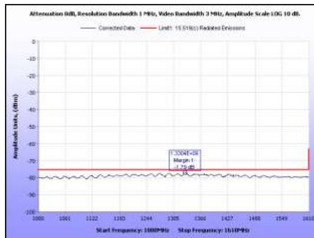
Plot 33. Radiated Emissions, 1 GHz – 1.61 GHz, BG6
