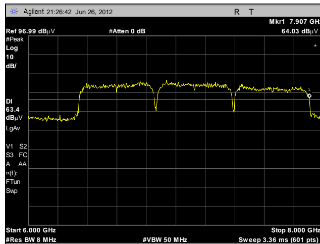
Plot 11. UWB Bandwidth, F_h , BG3
