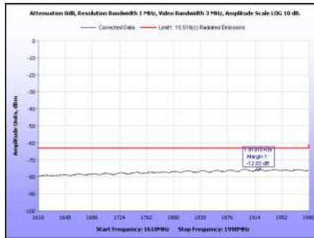
Plot 26. Radiated Emissions, 1.61 GHz – 1.99 GHz, BG3
