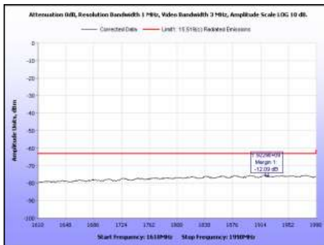
Plot 34. Radiated Emissions, 1.61 GHz – 1.99 GHz, BG6
