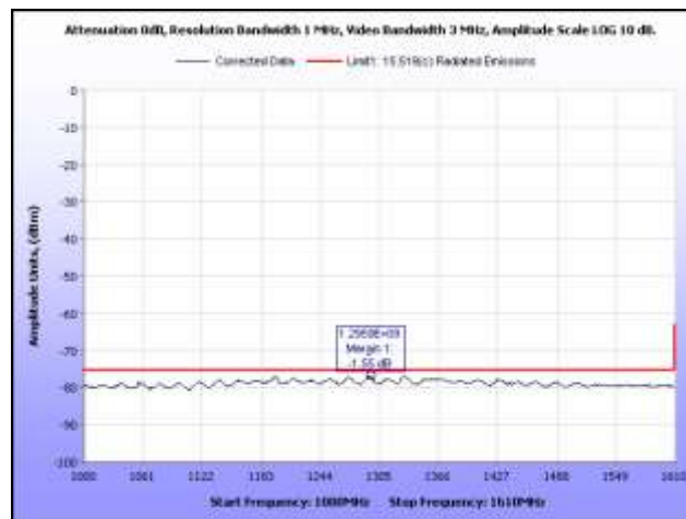
Plot 25. Radiated Emissions, 1 GHz – 1.61 GHz, BG3
