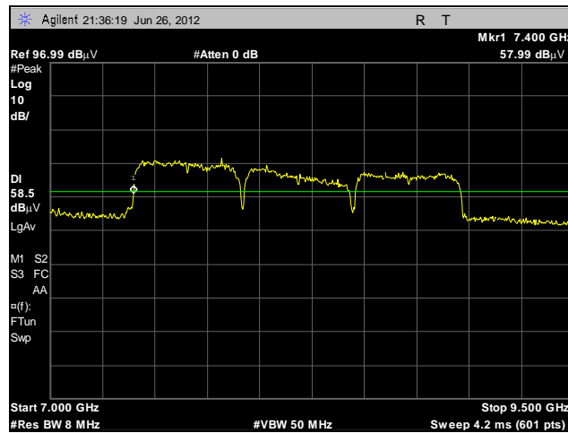
Plot 13. UWB Bandwidth, F_l , BG6
