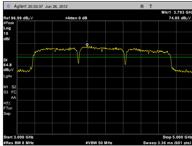
Plot 6. UWB Bandwidth, F_m , BG1
