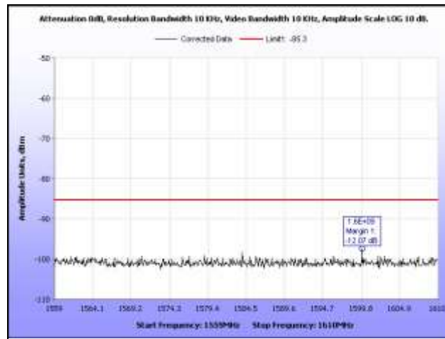
Plot 42. Radiated Emissions, 1.559 GHz – 1.61 GHz, GPS Band, BG3
