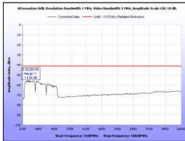
Plot 20. Radiated Emissions, 3.1 GHz – 10.6 GHz, BG1
