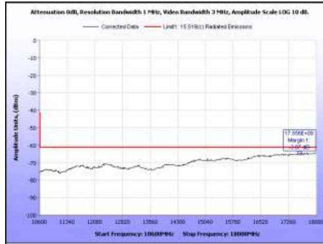
Plot 21. Radiated Emissions, 10.6 GHz – 18 GHz, BG1
