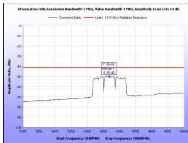
Plot 28. Radiated Emissions, 3.1 GHz – 10.6 GHz, BG3
