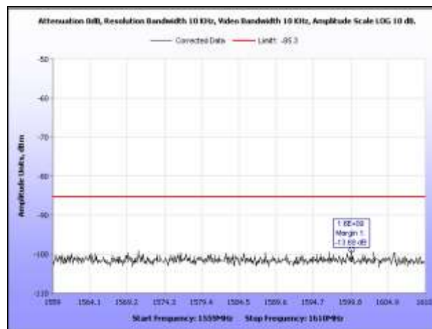
Plot 40. Radiated Emissions, 1.559 GHz – 1.61 GHz, GPS Band, BG1
