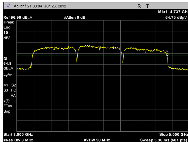
Plot 8. UWB Bandwidth, F_h , BG1
