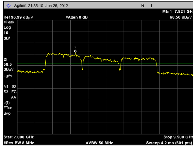
Plot 12. UWB Bandwidth, F_m , BG6
