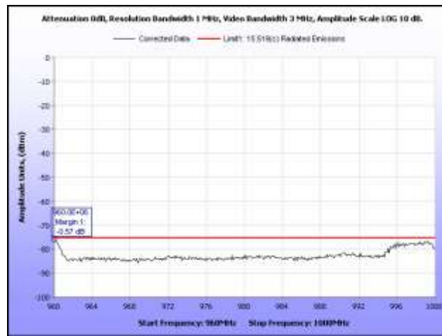
Plot 16. Radiated Emissions, 960 MHz – 1 GHz, BG1
