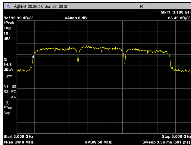
Plot 7. UWB Bandwidth, F_i , BG1
