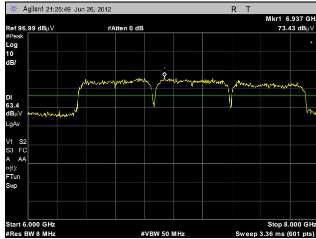
Plot 9. UWB Bandwidth, F_m , BG3
