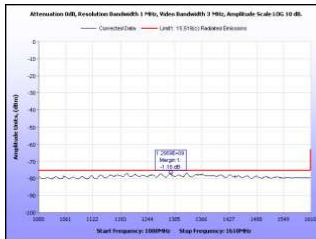
Plot 17. Radiated Emissions, 1 GHz – 1.61 GHz, BG1
