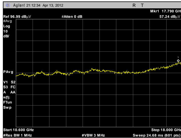
Plot 28. Radiated Emissions, 10.6 GHz – 18 GHz, BG3
