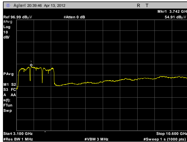
Plot 19. Radiated Emissions, 3.1 GHz – 10.6 GHz, BG1
