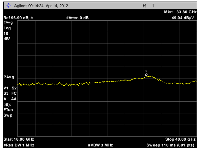
Plot 37. Radiated Emissions, 18 GHz – 40 GHz, BG6
