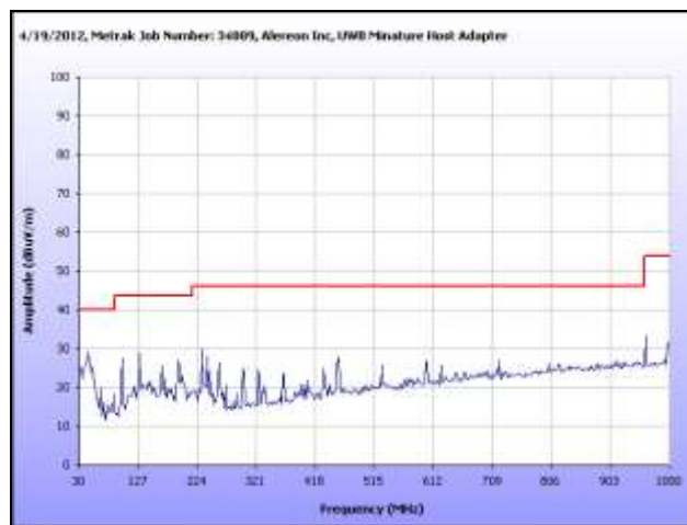
Plot 13. Radiated Emissions, 30 MHz – 1 GHz, BG3
