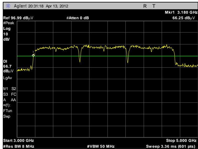
Plot 4. UWB Bandwidth, F_l , BG1
