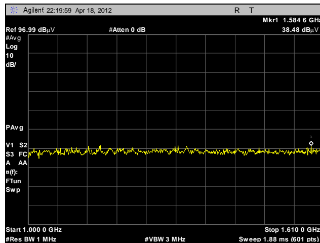
Plot 32. Radiated Emissions, 1 GHz – 1.61 GHz, BG6
