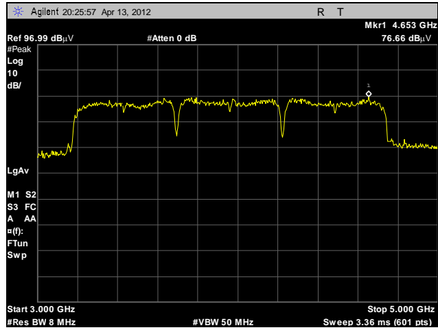
Plot 3. UWB Bandwidth, F_m , BG1
