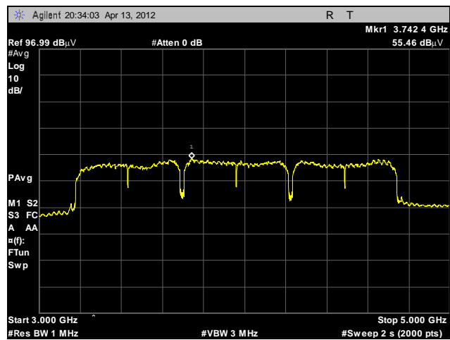
Plot 22. Radiated Emissions, Field Strength, BG1
