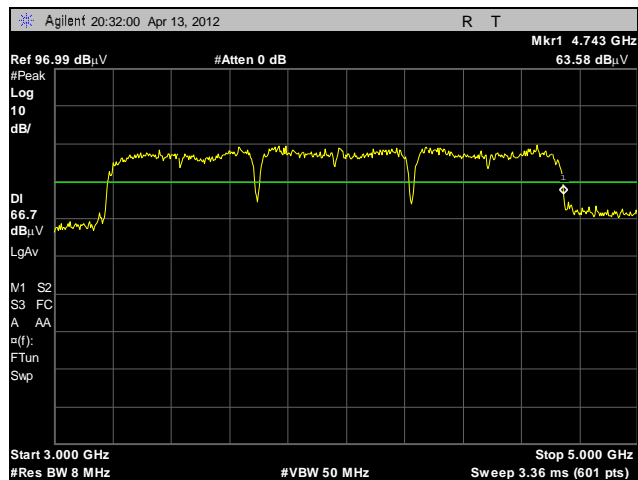
Plot 5. UWB Bandwidth, F_h , BG1
