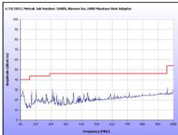
Plot 14. Radiated Emissions, 30 MHz – 1 GHz, BG6
