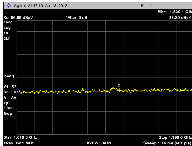
Plot 25. Radiated Emissions, 1.61 GHz – 1.99 GHz, BG3
