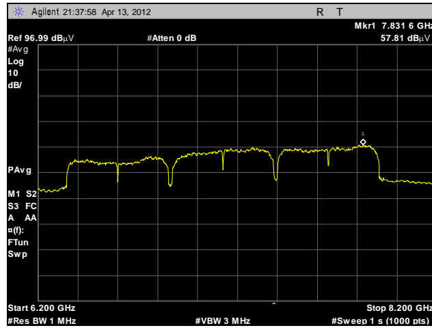
Plot 30. Radiated Emissions, Field Strength, BG3
