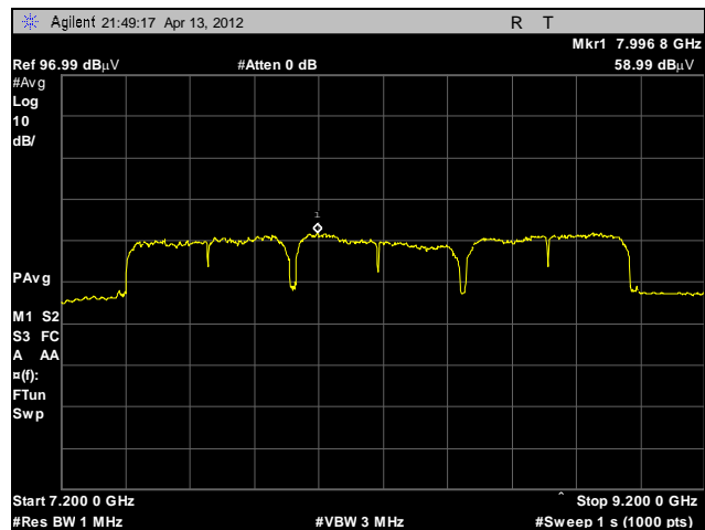
Plot 38. Radiated Emissions, Field Strength, BG6
