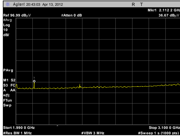
Plot 18. Radiated Emissions, 1.99 GHz – 3.1 GHz, BG1
