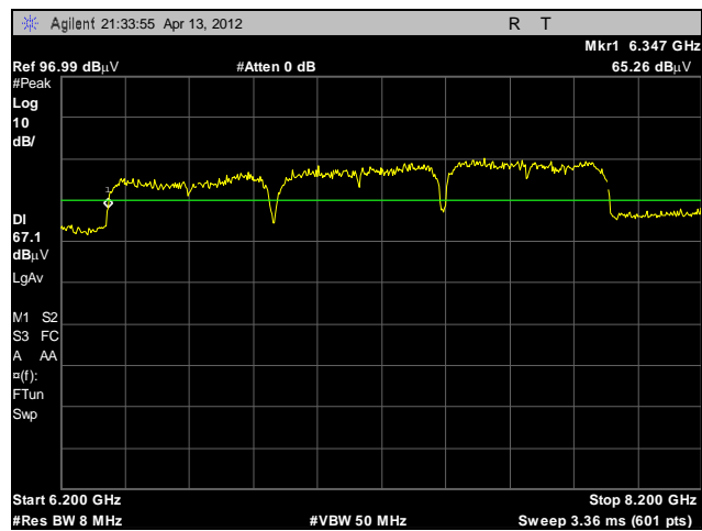
Plot 7. UWB Bandwidth, F_i , BG3
