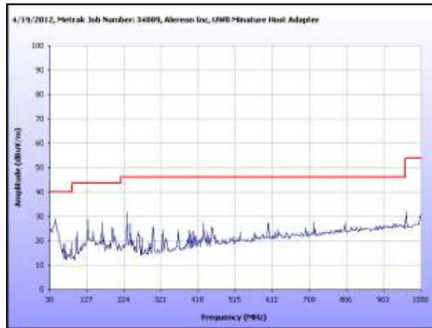
Plot 12. Radiated Emissions, 30 MHz – 1 GHz, BG1
