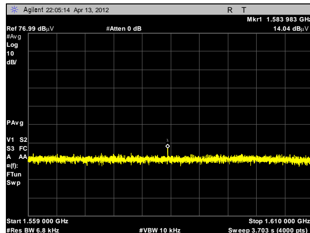
Plot 44. Radiated Emissions, 1.559 GHz – 1.61 GHz, GPS Band, BG6
