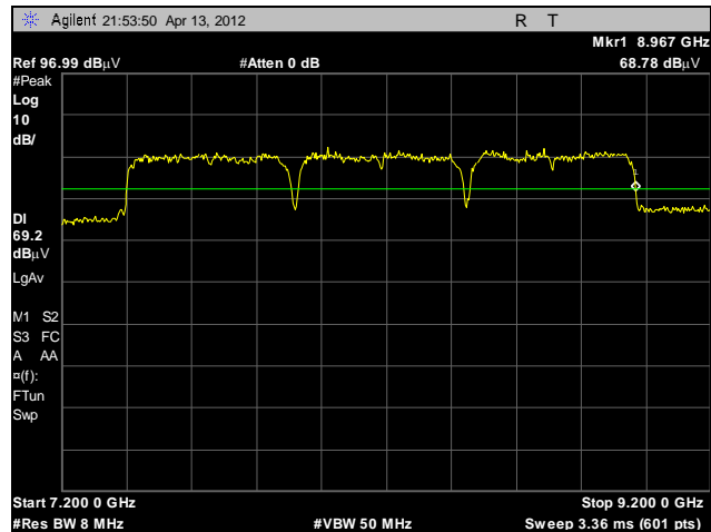
Plot 11. UWB Bandwidth, F_h , BG6
