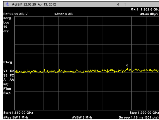
Plot 33. Radiated Emissions, 1.61 GHz – 1.99 GHz, BG6
