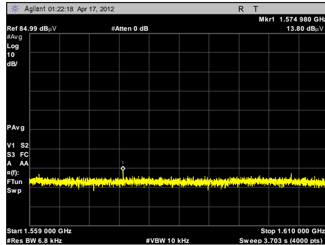
Plot 42. Radiated Emissions, 1.559 GHz – 1.61 GHz, GPS Band, BG3
