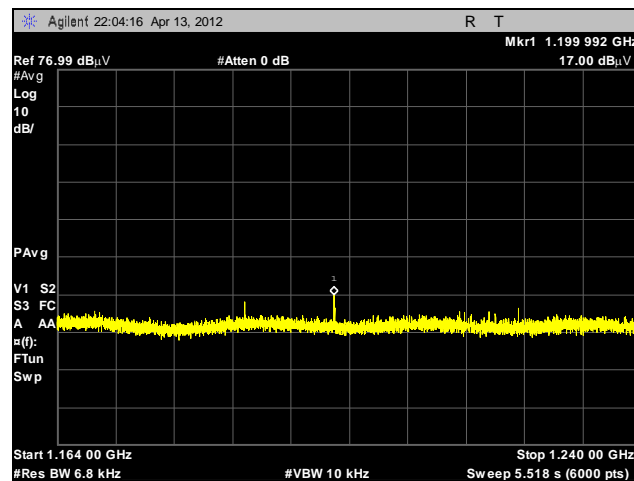
Plot 43. Radiated Emissions, 1.164 GHz – 1.24 GHz, GPS Band, BG6
