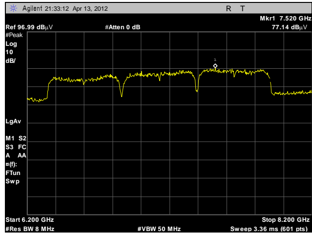
Plot 6. UWB Bandwidth, F_m , BG3
