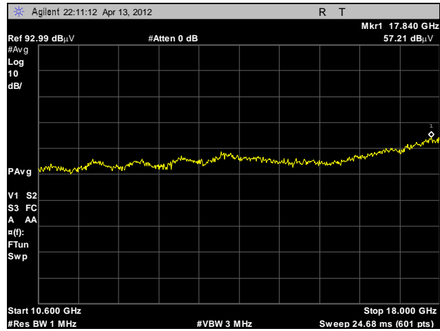
Plot 36. Radiated Emissions, 10.6 GHz – 18 GHz, BG6
