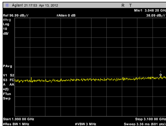
Plot 26. Radiated Emissions, 1.99 GHz – 3.1 GHz, BG3
