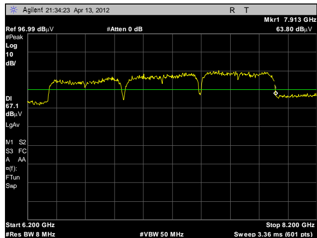
Plot 8. UWB Bandwidth, F_h , BG3
