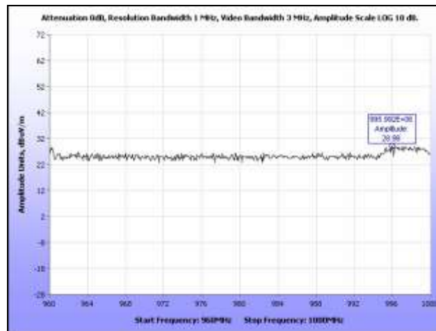
Plot 23. Radiated Emissions, 960 MHz – 1 GHz, BG3
