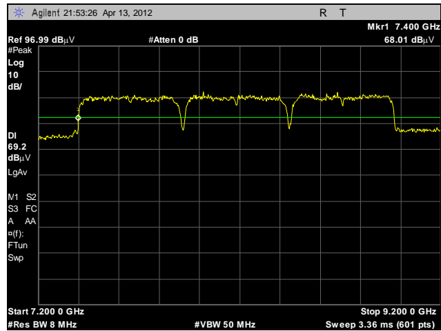
Plot 10. UWB Bandwidth, F_l , BG6
