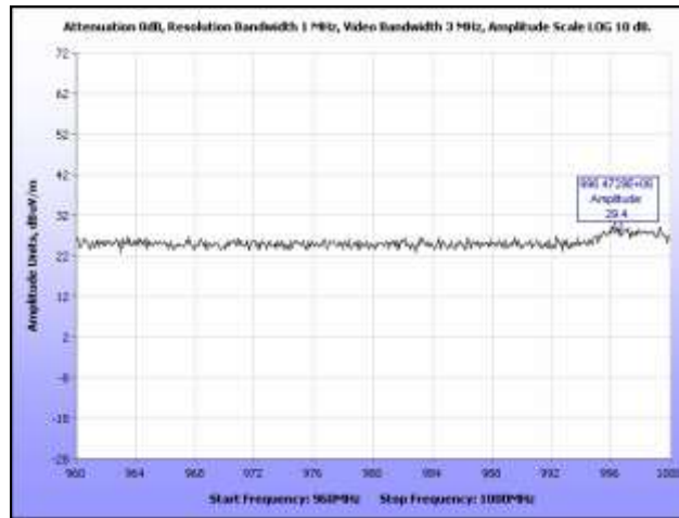
Plot 15. Radiated Emissions, 960 MHz – 1 GHz, BG1
