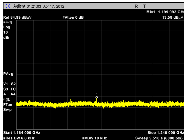
Plot 41. Radiated Emissions, 1.164 GHz – 1.24 GHz, GPS Band, BG3
