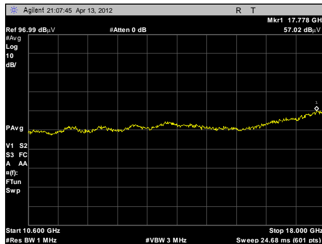
Plot 20. Radiated Emissions, 10.6 GHz – 18 GHz, BG1
