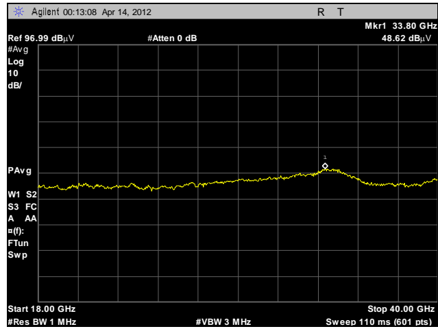
Plot 21. Radiated Emissions, 18 GHz – 40 GHz, BG1
