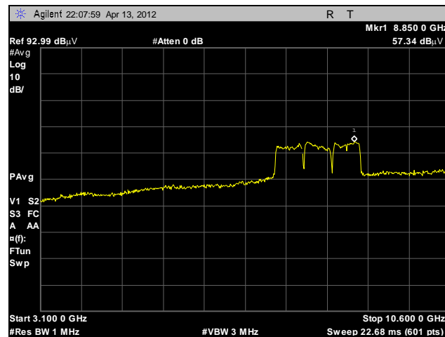
Plot 35. Radiated Emissions, 3.1 GHz – 10.6 GHz, BG6
