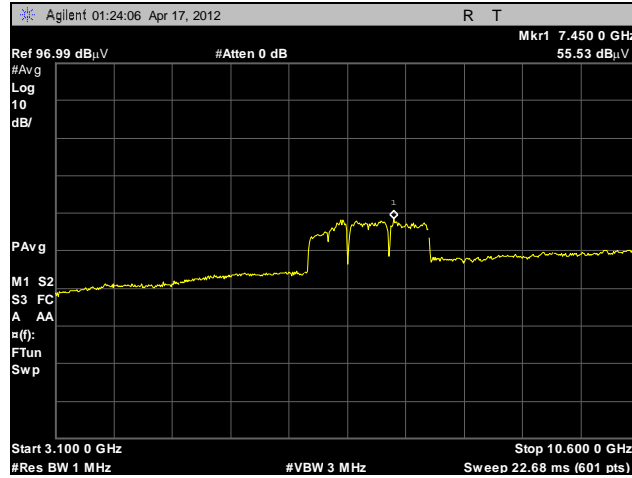
Plot 27. Radiated Emissions, 3.1 GHz – 10.6 GHz, BG3
