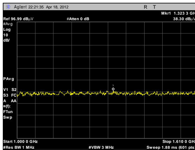
Plot 16. Radiated Emissions, 1 GHz – 1.61 GHz, BG1
