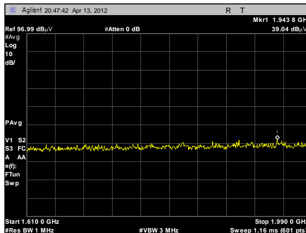
Plot 17. Radiated Emissions, 1.61 GHz – 1.99 GHz, BG1
