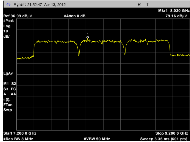
Plot 9. UWB Bandwidth, F_m , BG6
