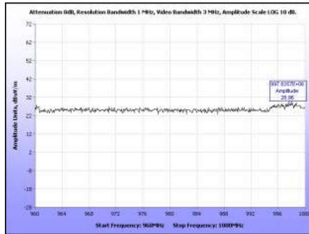
Plot 31. Radiated Emissions, 960 MHz – 1 GHz, BG6
