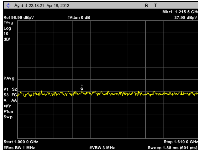
Plot 24. Radiated Emissions, 1 GHz – 1.61 GHz, BG3
