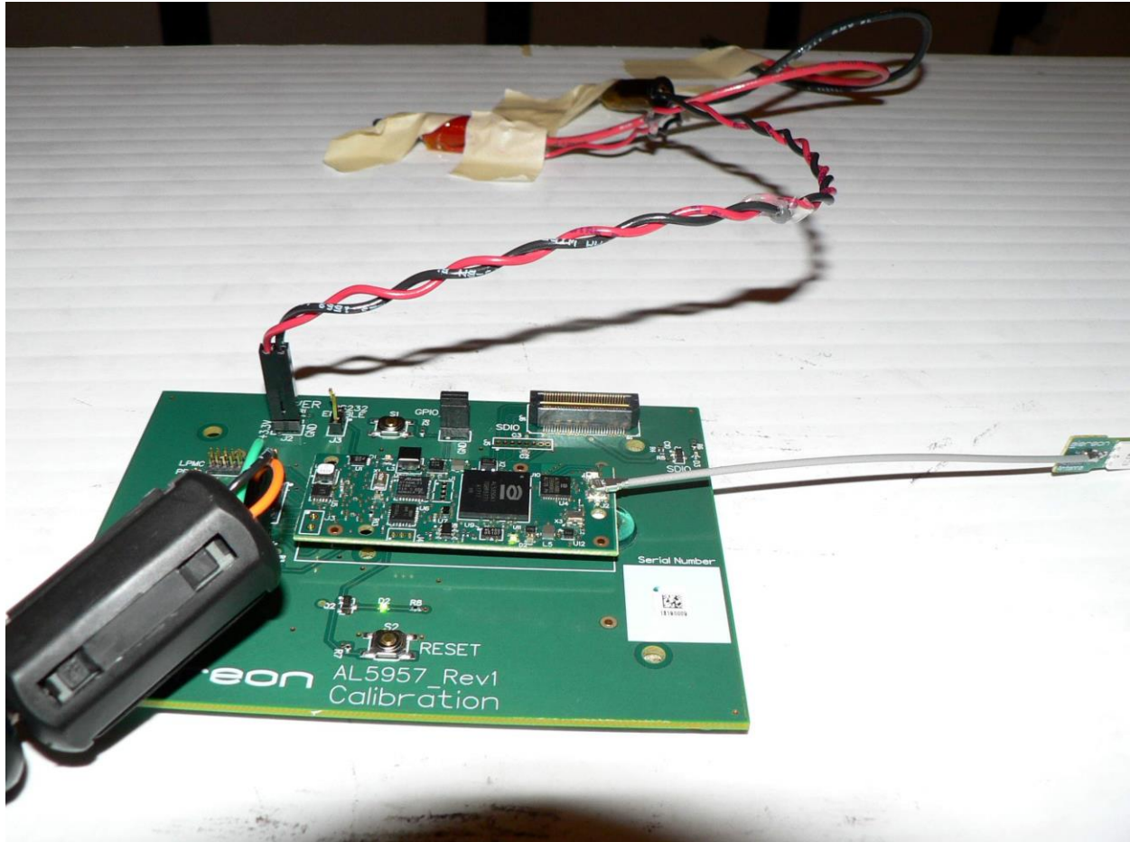
Camouflage TX Spurious Setup
