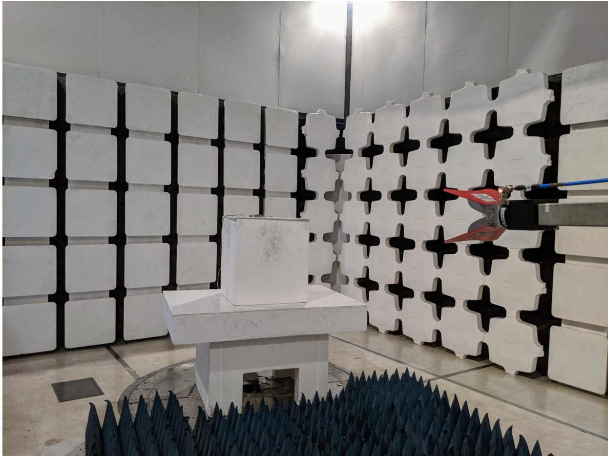
Emissions 1GHz - 18GHz
