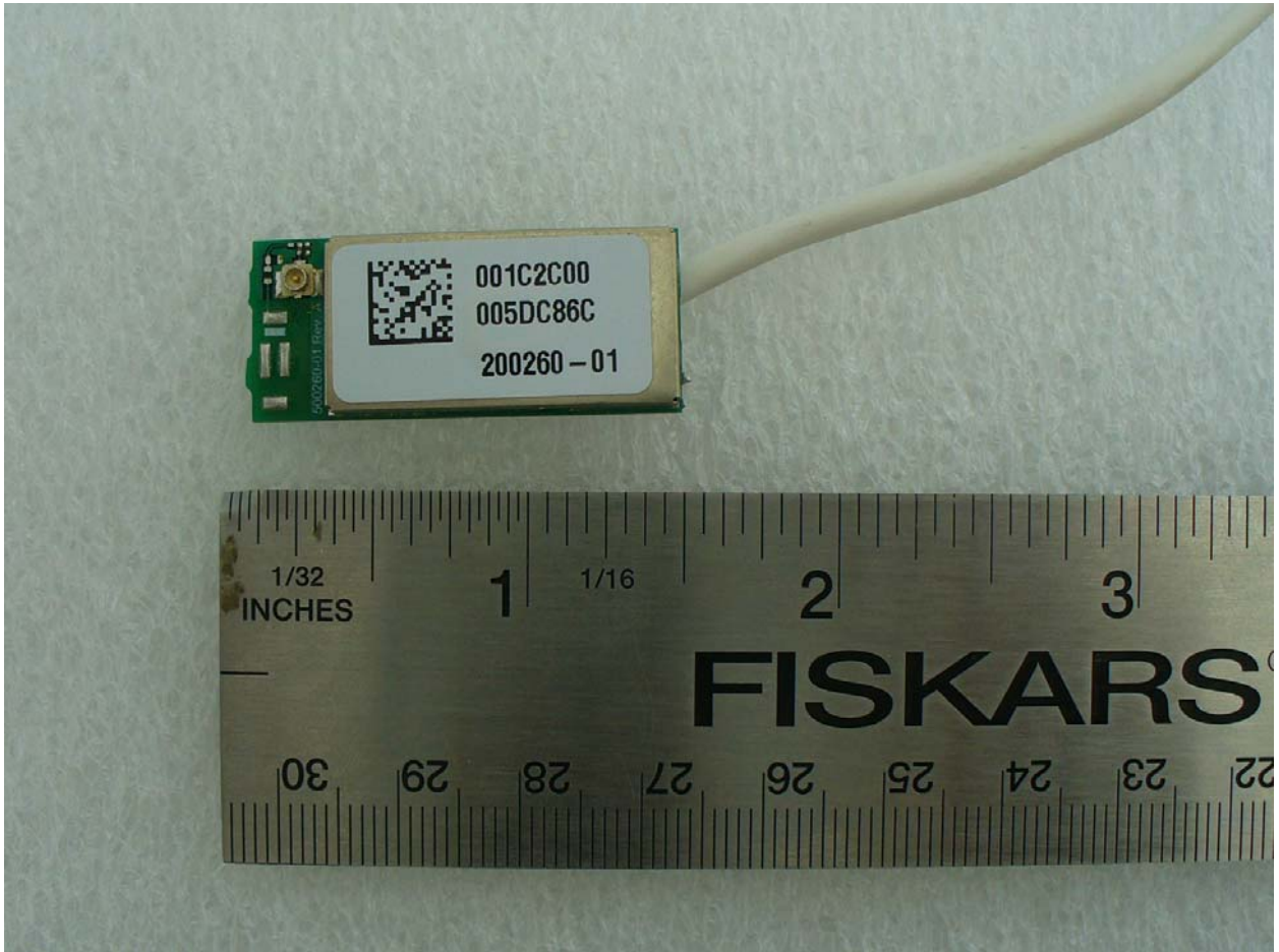
Figure 1: Top View (with shielding)
