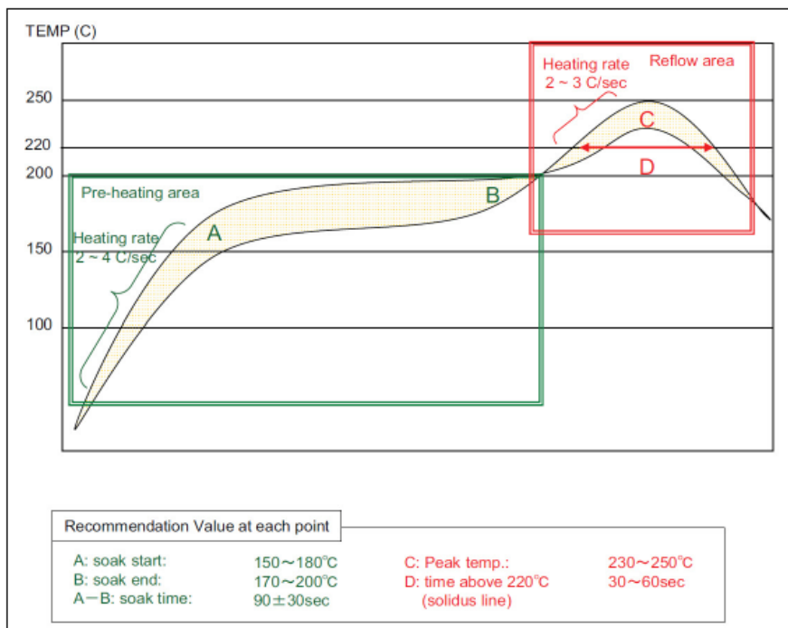
Figure 1.8: Reflow Profile Graph
