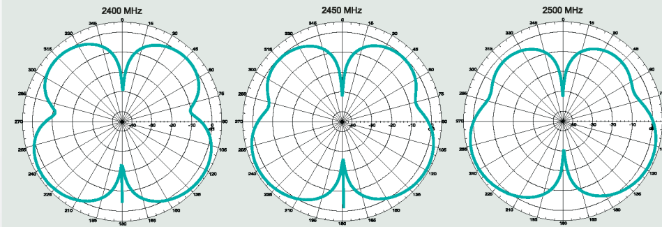
Figure 1.4: Pulse W1027 Antenna Gain Performance
