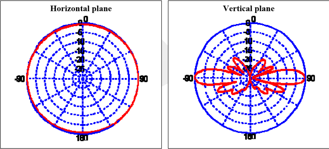
Figure 1.7: Pulse RO2408NF Antenna Gains Performance
