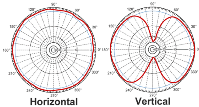
Figure 1.3: HyperLink Technologies HG2405RD-RSP Antenna Gain Performance
