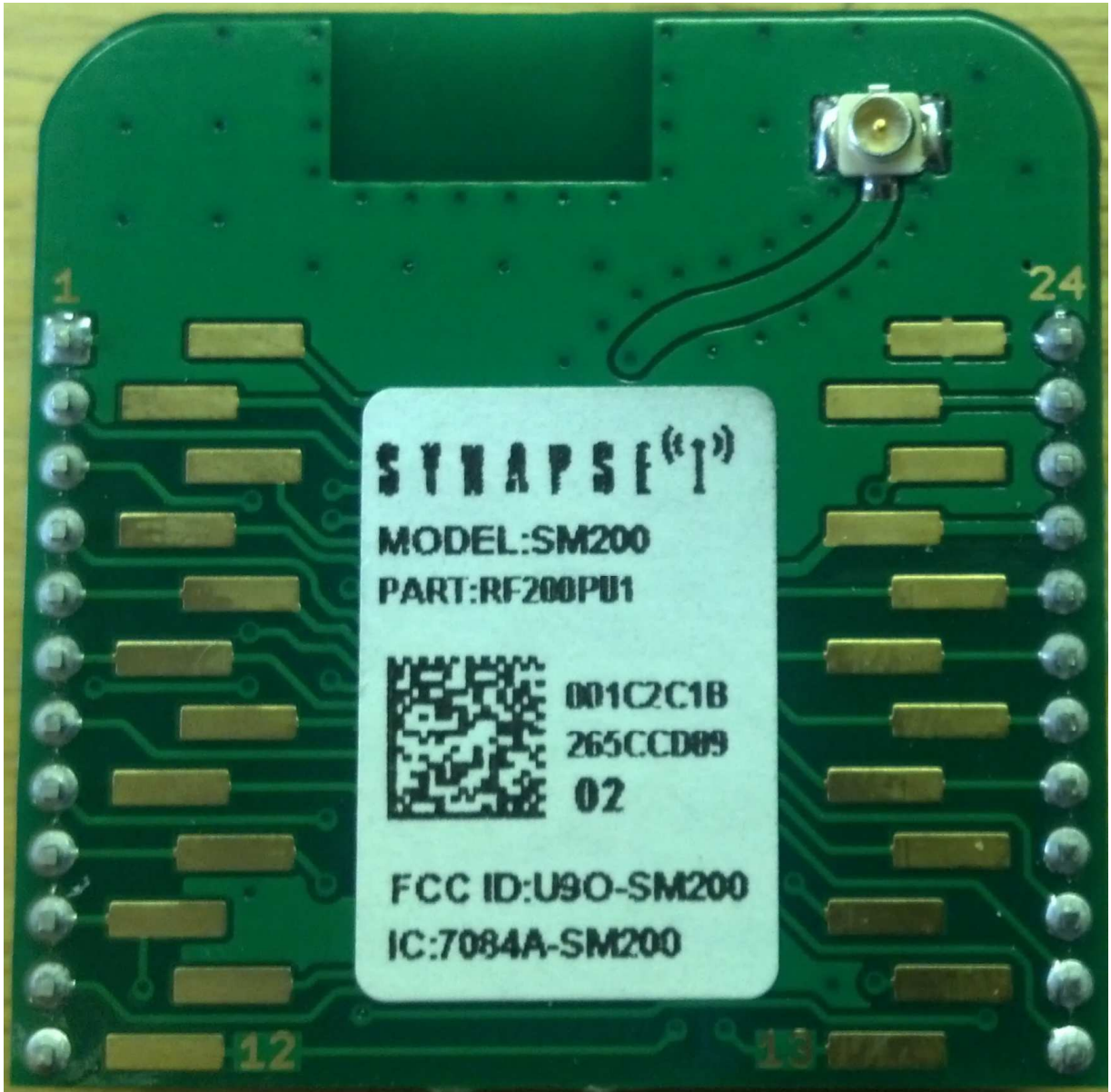
Figure 4: Sample Label & Placement – RF200PU1
