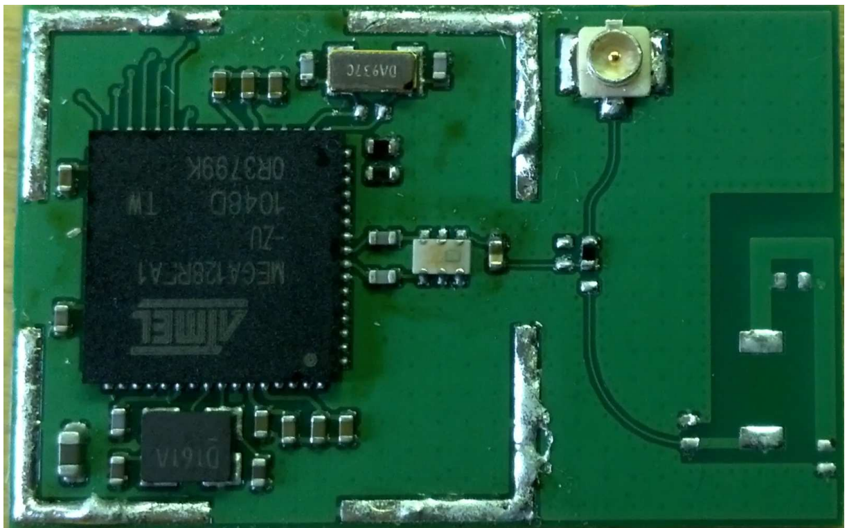
Figure 2: Internal Photo – SM200PU1
