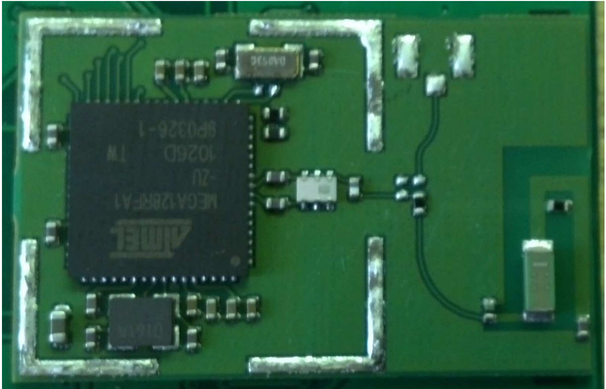
Figure 1: Internal Photo – SM200P81
