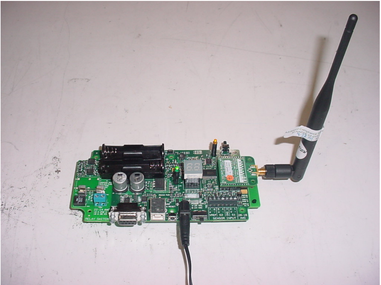
Figure 1: Test Setup – Radiated Emissions - RSMA
