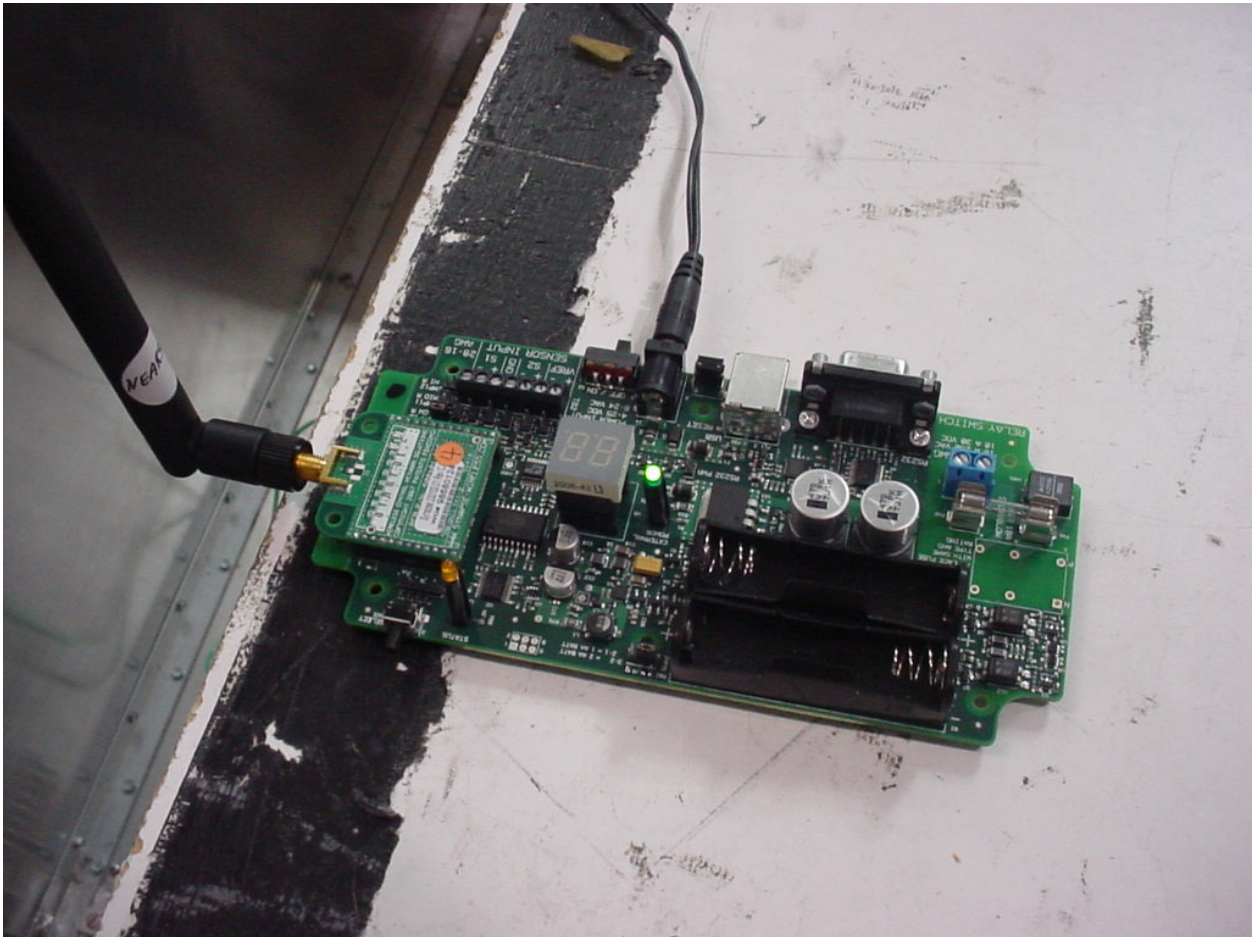
Figure 4: Test Setup – AC Power Line Conducted Emissions – RSMA
