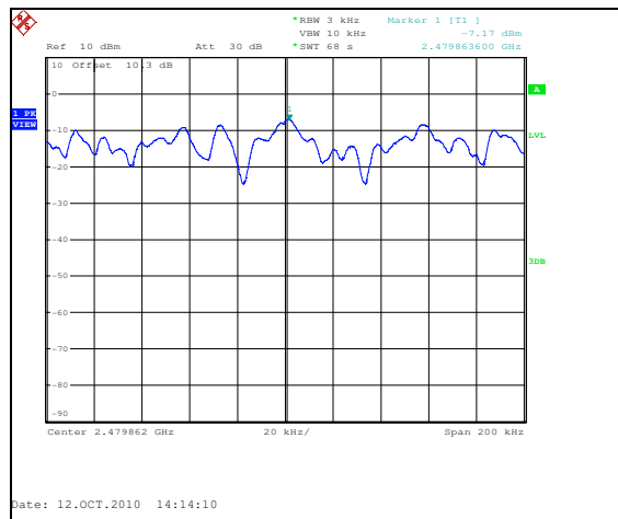
Figure 7.7.2-4: Power Spectral Density Plot – 2480MHz
