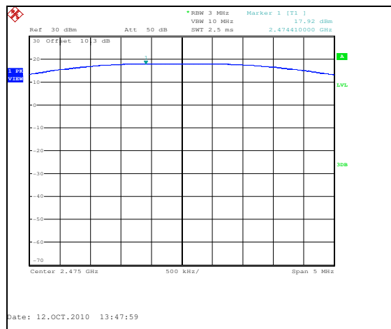
Figure 7.5.2-3: Output power – 2475MHz
