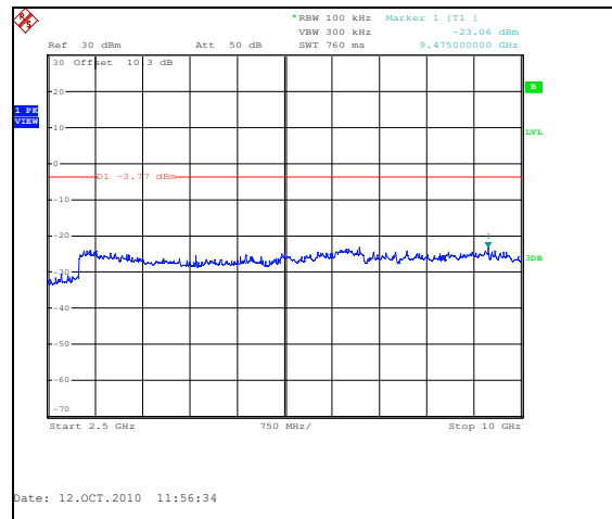
Figure 7.6.2.2-2: 2.5 GHz – 10 GHz – 2405MHz
