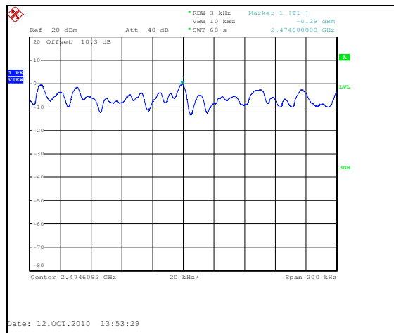
Figure 7.7.2-3: Power Spectral Density Plot – 2475MHz
