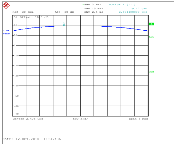
Figure 7.5.2-1: Output power – 2405MHz
