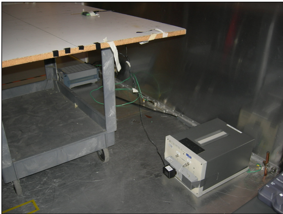
Figure 2: Conducted Emissions
