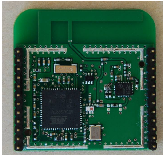
Figure 4: Bottom View - without shielding (RF200APF1)
