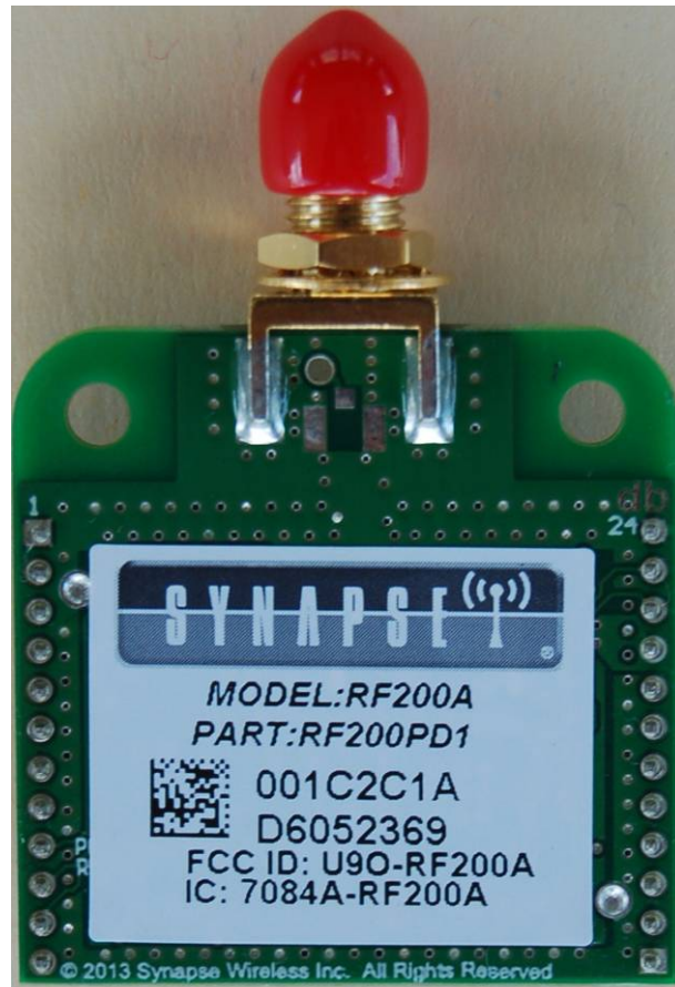
Figure 1: Top View (RF200APD1)
