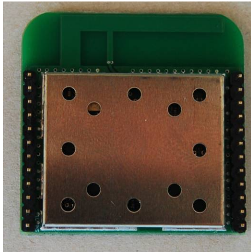
Figure 4: Bottom View - with shielding (RF200APF1)
