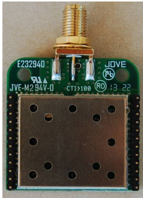
Figure 2: Bottom View - with shielding (RF200APD1)
