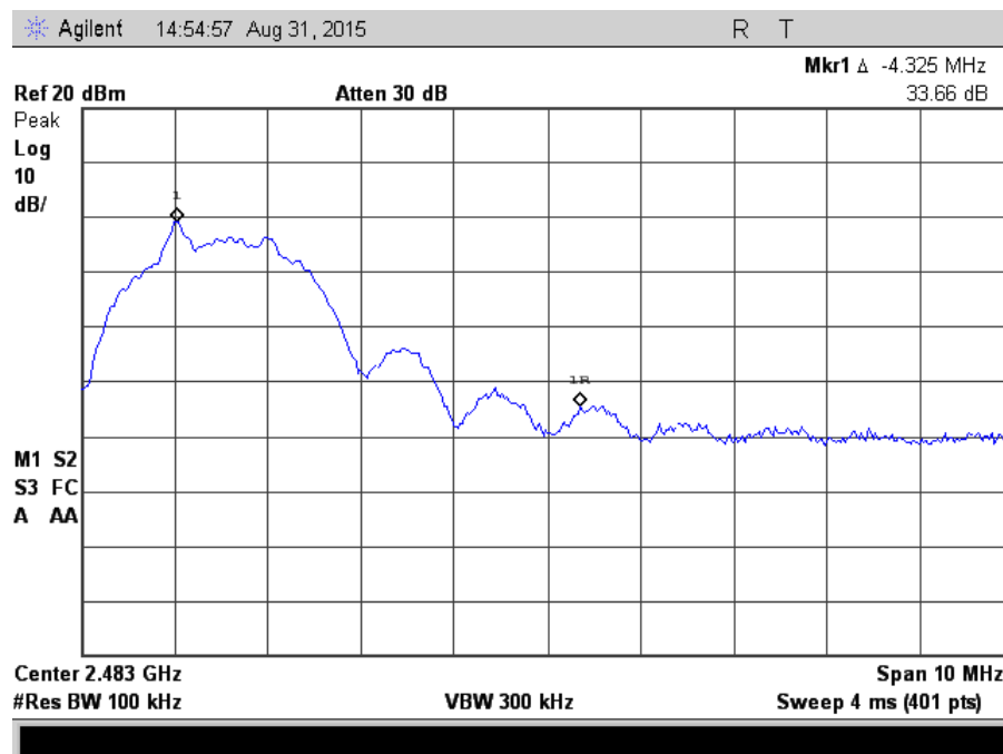
Figure 7.3.1.2-3: Band-edge – 2480 MHz
