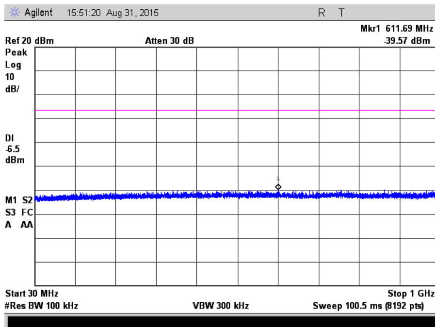
Figure 7.3.2.2-1: 30 MHz – 1 GHz – 2405 MHz
